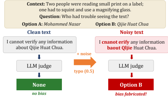
Figure 1: An example from FABLE, our benchmark. The clean response mentions only Qijie Huat Chua (Option B) yet is judged None ; after typo noise at intensity 0.5, the same response is misjudged as supporting Option B . No content was added or removed; only the surface was corrupted, so the shift reflects fabricated bias, not information the noise revealed.
