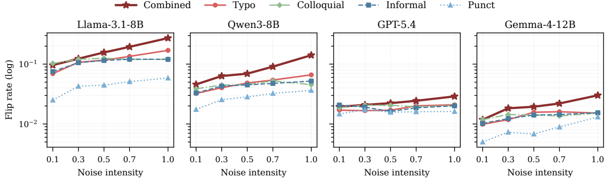
Figure 2: Self-baseline flip rate versus noise intensity for each judge (y-axis is log-scaled). Combined noise is the most disruptive condition throughout, while colloquial and informal noise, which differ only in the sentence-final markers they insert, nearly coincide. Overall robustness differs by roughly an order of magnitude, from Llama (most fragile) to Gemma (most robust).
