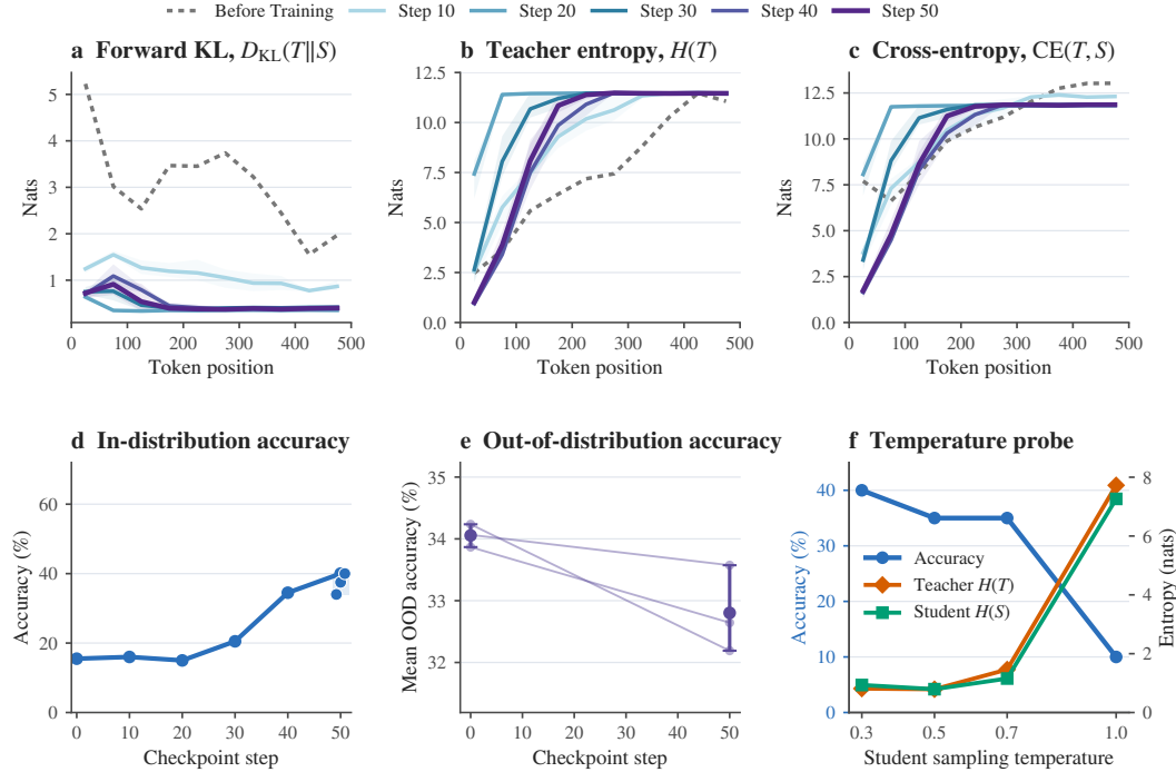
Figure 22: Science OnPD forward-KL dynamics. (a)–(c): token-position profiles at initialization (dotted grey) and every 10 training steps through step 50 (solid lines: three-seed means; shading: min–max ranges). (d): held-out accuracy for seed 42, with all three repeats at step 50. (e): OOD accuracy for individual seeds, with mean markers and min–max bars at initialization and step 50. (f): accuracy and teacher/student entropy when re-sampling the seed-42 checkpoint-50 model on the same 20 prompts at different temperatures.
