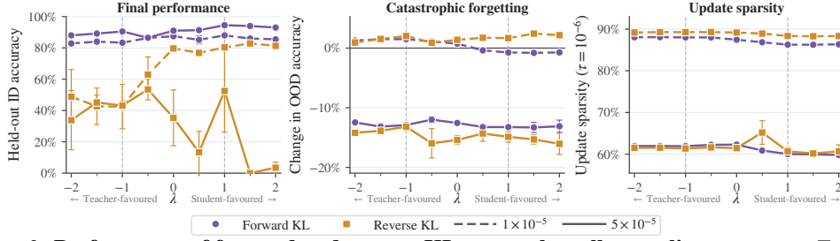
Figure 3: Performance of forward and reverse KL across the rollout-policy spectrum. Forward KL maintains strong final performance across the spectrum, whereas reverse KL varies substantially. Rollout policy has comparatively little effect on catastrophic forgetting or update sparsity. Points show means over N = 3 seeds; error bars denote SEM.
