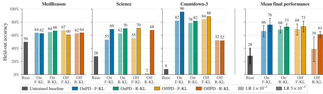
Figure 13: Comparison of the effectiveness of OnPD and OffPD training for Qwen2.5-1.5B. Dataset panels report mean held-out accuracy over N = 3 repeats; error bars show SEM. The right-most panel shows the average across the nine runs. Across the evaluated settings, KL direction appears to have a larger effect on final performance than rollout policy, with forward KL outperforming reverse KL on average.
