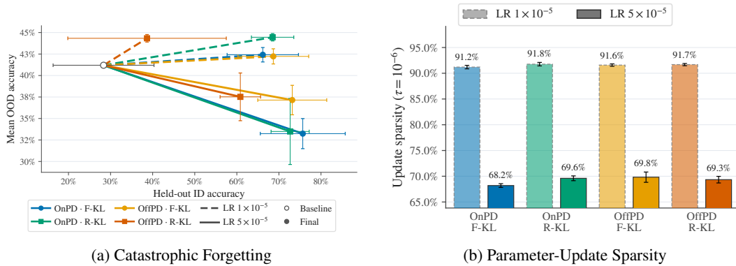
Figure 14: Catastrophic forgetting and parameter-update sparsity for Qwen2.5-1.5B. Similarly as for Llama3.2-1B, we observe that for Qwen2.5-1.5B learning rate is a stronger predictor of the degree of catastrophic forgetting and the parameter-update sparsity than the rollout policy. Left: The mean OOD accuracy consistently decreases over the course of training when the larger learning rate of 5 \times 10^{-5} is used, but increases when the smaller learning rate is used instead. OffPD does not lead to stronger forgetting in any of the conditions. Right: Similarly, parameter-update sparsity does not vary significantly between the rollout policies, but depends strongly on the learning rate. For both figures, error bars mark SEM computed over the three datasets.
