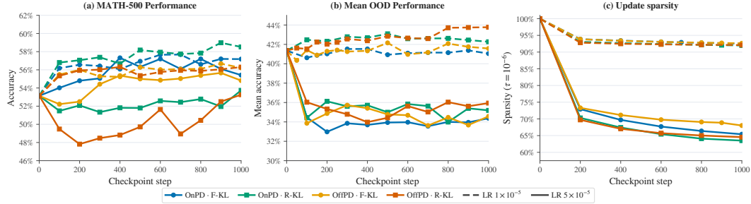
Figure 11: MATH-500 performance throughout training. Accuracy is evaluated every 100 optimization steps using ten generations per problem. Performance generally improves beyond the untrained baseline, although the optimal checkpoint varies considerably across conditions. The lower learning rate produces more stable learning trajectories, while the larger learning rate is particularly unstable with reverse KL. Looking at catastrophic forgetting and parameter-update sparsity, differences between OnPD and OffPD remain comparatively modest relative to the effects of learning rate and KL direction.
