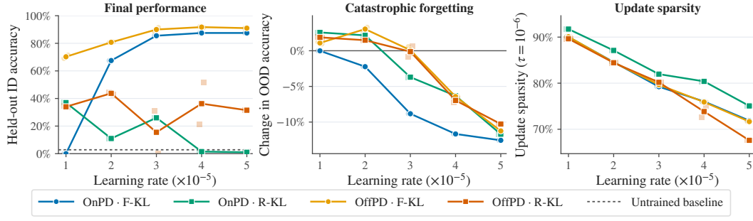
Figure 8: The effect of learning-rate without gradient clipping. Removing clipping reveals a substantial difference in final performance between forward and reverse KL, with reverse KL suffering from unstable training, while learning rate remains the dominant determinant of forgetting and parameter-update sparsity.
