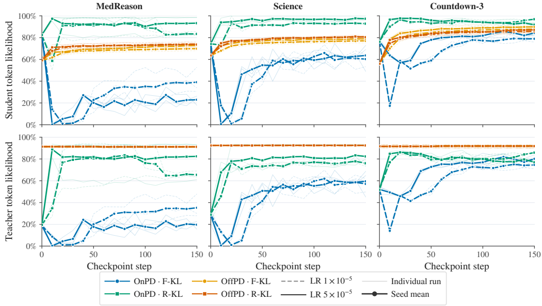
Figure 21: Teacher and student likelihoods on the trajectories generated during OnPD and OffPD training. Both the teacher and student likelihoods were computed at temperature 1.0.
