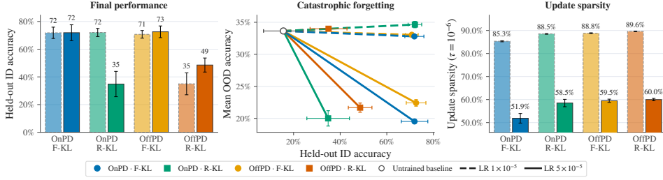
Figure 1: Comparison of OnPD and OffPD across three reasoning tasks. Held-out ID accuracy in the left and middle panels is averaged across MedReason, Science, and Countdown-3. Per-dataset results are reported in Figure 20. Error bars show SEM computed over N = 3 seeds.
