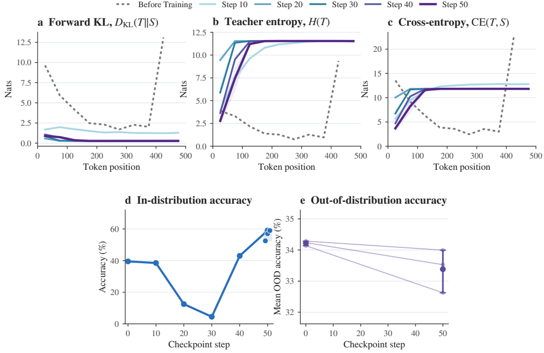
Figure 23: MedReason OnPD forward-KL dynamics. (a)–(c): token-position profiles of forward KL, teacher entropy, and cross-entropy. (d)–(e): held-out MedReason and OOD accuracy. Plotting conventions match Figure 22.
