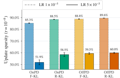
Figure 18: Parameter-update sparsity with a smaller threshold. Each bar pools the three datasets and N = 3 repeats per dataset; error bars show SEM across the nine runs. Learning rate, more than rollout policy, determines sparsity of updates.
