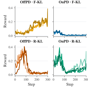
Figure 6: RLVR rewards on Countdown-4 when starting from distillation checkpoints trained with LR 1 \times 10^{-5} ; each curve corresponds to a distillation seed.
