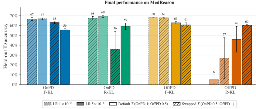
Figure 25: Generation-temperature ablation on MedReason. Modifying the generation temperature does not affect the best performance achieved by either OnPD or OffPD. Error bars mark the SEM over N = 3 seeds.
