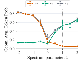
Figure 4: Likelihood in the rollout-policy spectrum.
