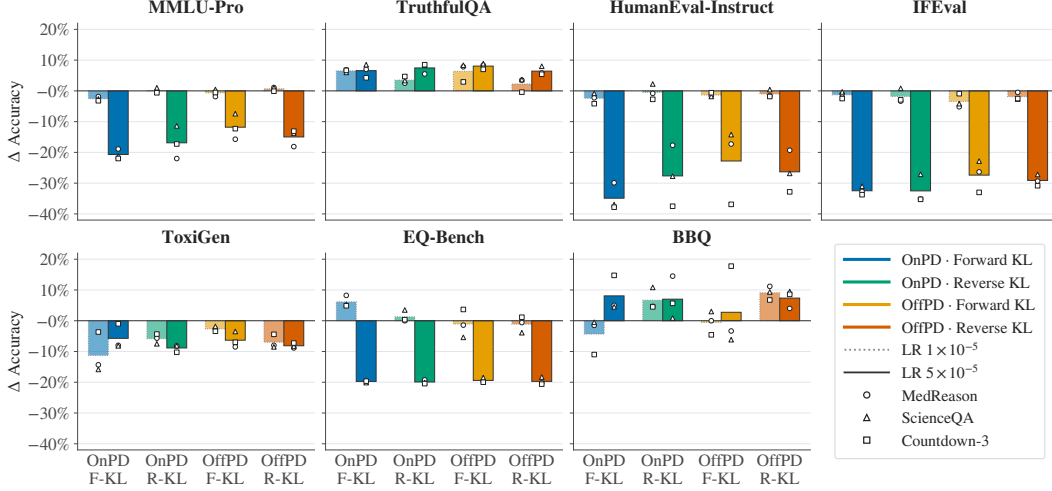
Figure 17: Per-benchmark changes in out-of-distribution performance. Each panel reports the change from the untrained student baseline to the final distilled checkpoint on one OOD benchmark. Bars average repeated runs within each training task and then weight MedReason, Science, and Countdown-3 equally. White markers show the corresponding training-task means.
