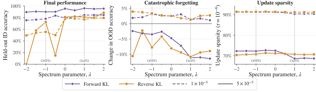
Figure 15: Sensitivity of Qwen2.5-1.5B to the rollout policy. Results at checkpoint 150 across the contrastive-decoding spectrum, using seed 42. The performance of forward-KL is robust to the rollout policy, while the performance of reverse-KL degrades sharply under teacher-favoured rollouts. Consistent with previous findings, larger learning rates amplify forgetting, particularly for student-favoured rollouts, while also producing denser parameter updates.
