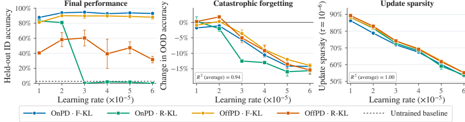
Figure 2: The effect of learning rate on Countdown-3. Forgetting increases and update sparsity decreases with the learning rate under both rollout policies. Points report means over N = 3 seeds; error bars show SEM.
