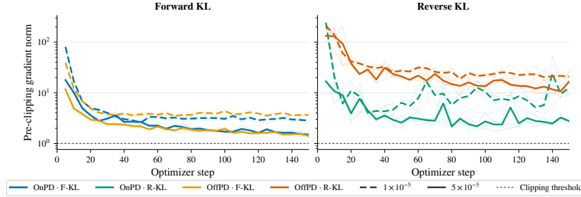
Figure 7: Gradient clipping is active throughout Countdown-3 training. We show the global gradient norm before clipping for the Countdown-3 runs which use gradient clipping, with thin lines denoting individual seeds and thick lines their mean across three seeds. The horizontal line marks the clipping threshold of 1.0. Every recorded norm exceeds this threshold, demonstrating that clipping rescales the gradients at every logged optimization step. Reverse KL produces substantially larger and more variable gradient norms than forward KL, including pronounced early spikes, supporting the role of clipping in stabilising reverse-KL training.
