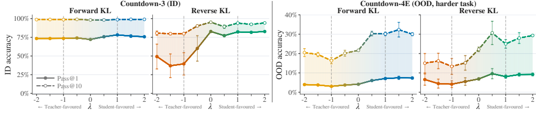
Figure 5: Output coverage and generalisation along the rollout-policy spectrum. While in-distribution forward KL leads to better output coverage, when generalising to harder tasks we can see a clear benefit of using on-policy data. Error bars show SEM across three seeds. The easier Countdown-3 uses T = 1 , while the more difficult Countdown-4E uses T = 0.5 .
