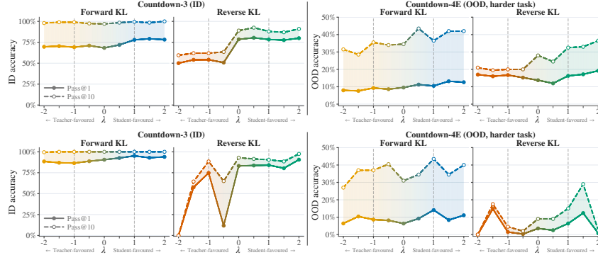
Figure 16: Output coverage and generalisation for Qwen2.5-1.5B. LR 1 \times 10^{-5} (top) and 5 \times 10^{-5} (bottom). Same plotting conventions as Figure 5.
