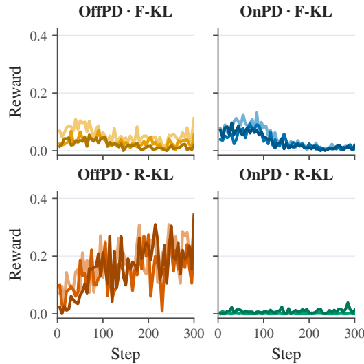
Figure 26: Countdown-4 RLVR rewards after distillation at LR 5 \times 10^{-5} ; each curve is a distillation seed.
