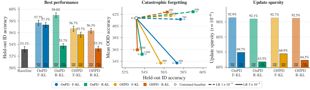
Figure 10: Math distillation results on MATH-500. We report the best MATH-500 performance attained during training, movement from the untrained baseline in ID–OOD space, and parameter-update sparsity at the corresponding selected checkpoint. In this regime, OnPD with reverse-KL outperforms other conditions. However, the learning rate still largely controls catastrophic forgetting and parameter-update sparsity. The performance of forward KL is also more robust to the changes in rollout policy and learning rate.
