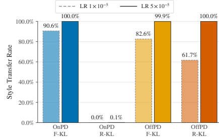
Figure 24: Style transfer from teacher to student model. OnPD with R-KL does not learn to generate traces in Spanish.
