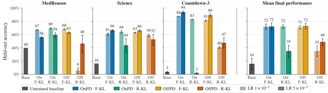
Figure 20: Breakdown of the final performance obtained on each dataset. We demonstrate a breakdown of the final performance after 150 steps of training, across the three datasets. Error bars denote SEM computed over N = 3 seeds.
