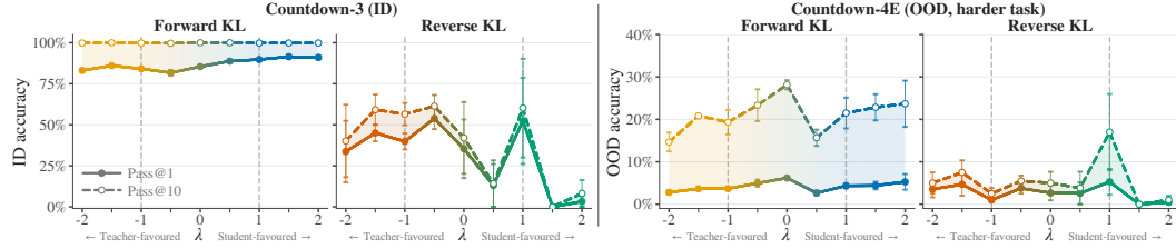
Figure 12: Output coverage and generalisation at LR 5 \times 10^{-5} for Llama3.2-1B. Same protocol and plotting conventions as Figure 5; means and SEM over three distillation checkpoints.
