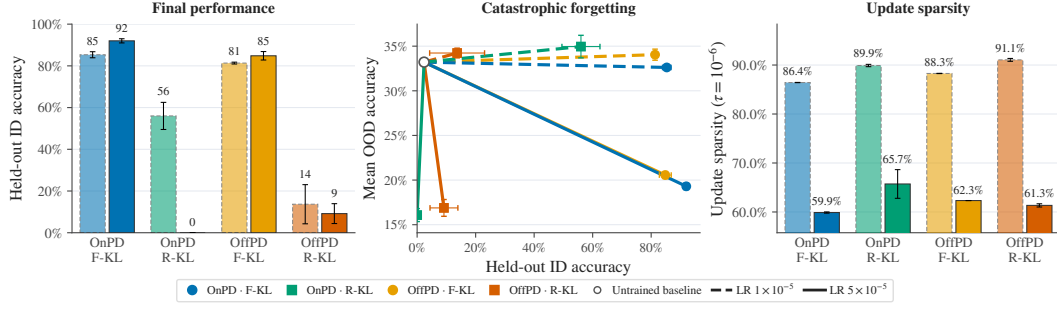
Figure 9: Performance after training with sampled KL. Error bars show SEMs computed over N = 3 seeds. Sampled-KL training exhibits the same qualitative trends as full-vocabulary KL. Forward KL achieves substantially higher and more robust final performance than reverse KL, while differences between OnPD and OffPD are comparatively limited. Catastrophic forgetting and update sparsity are governed primarily by the learning rate. These results indicate that replacing full-vocabulary KL with a single-sample gradient estimator does not materially alter our main conclusions regarding rollout policy, KL direction, and learning rate.
