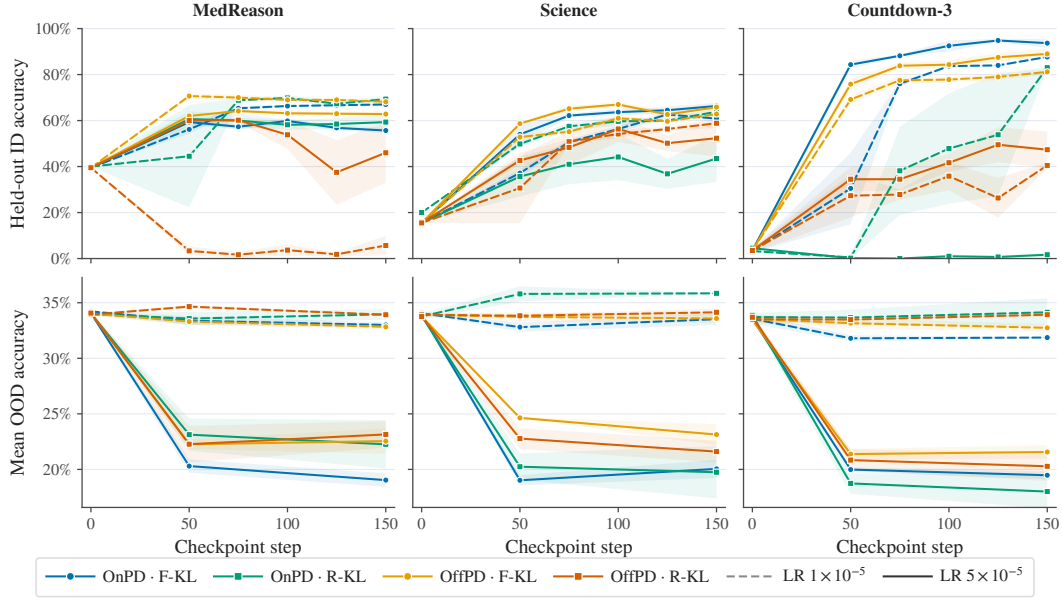
Figure 19: Learning and forgetting curves for the main runs on Llama3.2-1B-Instruct. We report the accuracy on the held-out test set of the training task (top row) and the mean accuracy over the out-of-distribution tasks (bottom row) over the course of training. We can observe that for the majority of the runs, the target task performance converges to a stable value after 150 optimisation steps. Additionally, most of the forgetting happens within the first 50 steps of training, with the OOD performance maintaining a relatively stable value at steps 50-150. The shading represents mean \pm one standard error of the mean (SEM) computed over three seeds.
