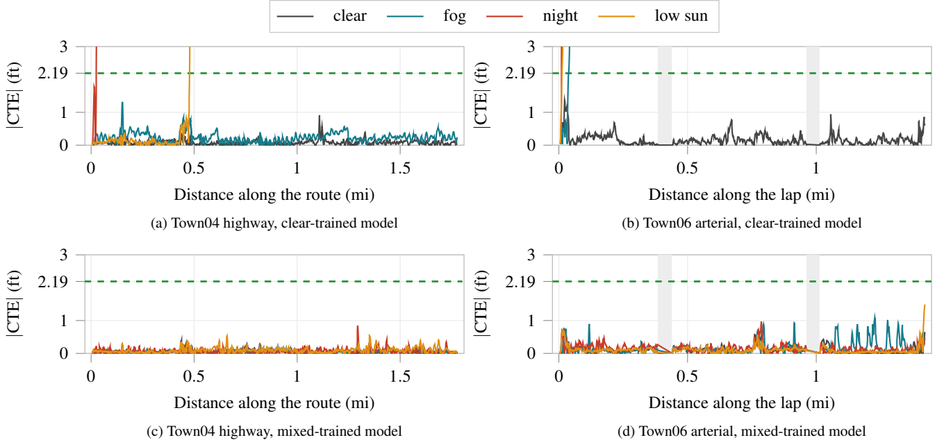
Figure 5: Cross-track error along the route against the 2.19 ft budget (dashed). Each trace stops the first time it passes 3 ft, and the gray bands are Town06’s two bridged intersections, which no policy steers.
