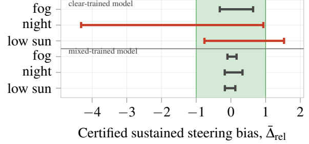
(a) Town04, six test cases, each bar the envelope of the two driven directions.
