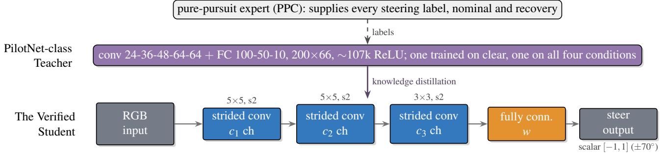
Figure 2: All four models share this topology, differing only in the widths tabulated in Table 1. Each is distilled from a PilotNet-class teacher trained on pure-pursuit labels, and only the student model is verified.
