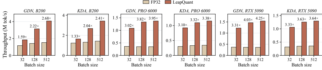
Figure 7: Kernel throughput of one linear attention layer.
