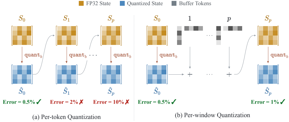
Figure 2: Per-token versus per-window quantization. Per-token quantization re-quantizes the full state after every update. Per-window quantization holds the quantized boundary state \hat{S}_0 fixed, buffers the p updates of the window in higher precision, and reconstructs the state from them; the full state is quantized only once per window, into \hat{S}_p .
