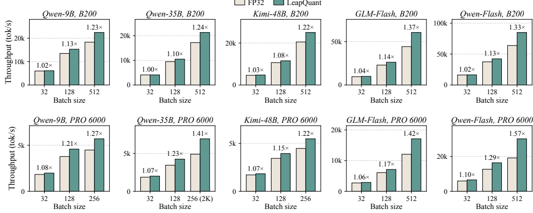
Figure 8: Decode-step throughput in vLLM at context length 4K. On the RTX PRO 6000, the largest batch size is 256 where 512 does not fit, and Qwen3.5-35B-A3B uses 2K instead of 4K at this batch size.
