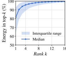
Figure 5: Energy of the top singular values in the Qwen3.5-9B model.
