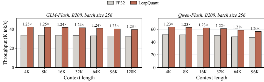
Figure 11: Decode-step throughput of the two sparse-attention models on the B200 at batch size 256 and long contexts.
