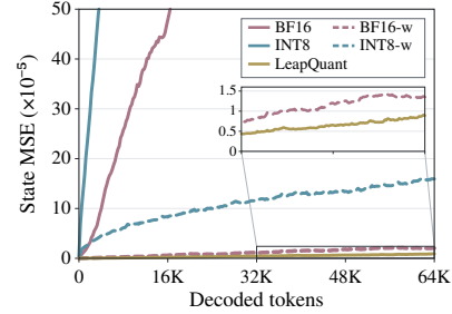
Figure 3: State MSE over 64K decoded tokens on PG-19 (Qwen3.5-9B); -w quantizes once per window.
