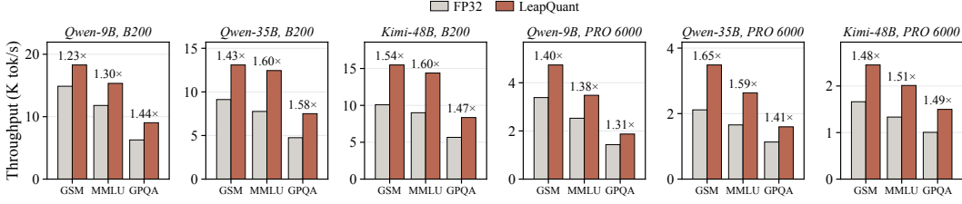
Figure 9: End-to-end inference throughput on different datasets.
