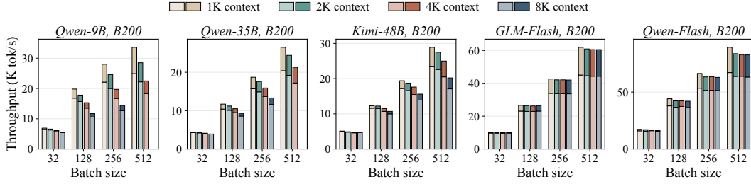
Figure 10: Decode-step throughput in vLLM on the B200 at context lengths 1K–8K. Each bar stacks the FP32 throughput (lighter) and the gain of LeapQuant (darker).
