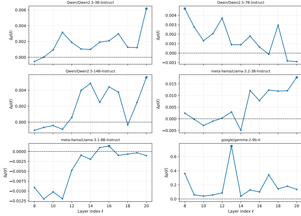
Figure 1: Per-model layer sweeps of \Delta\rho(\ell) on the comparative run. Each panel reports one model, with the selected best layer marked.
