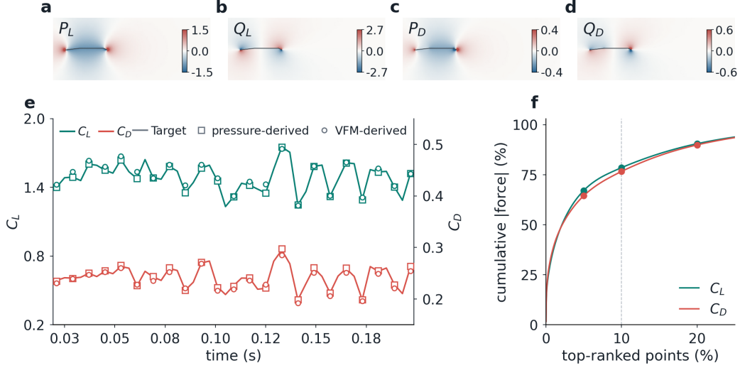
Figure 3: Physical basis for the VFM coupling, shown for (\theta_1, \theta_2) = (174.1^\circ, 155.0^\circ) at AoA = 12^\circ . (a–d) Panel-method coefficient fields P_L, Q_L, P_D, Q_D . (e) Lift and drag recovered on paired left/right ordinates from the target force record, the pressure integral on the target pressure field, and the VFM integral evaluated on the target velocity and mesh curl; the VFM mean absolute relative errors are 2.09% for C_L and 2.22% for C_D . (f) Cumulative absolute force contribution after ranking fluid points by local VFM magnitude. At the displayed input frame ( t = 0.073 s) the top 10% contributes approximately 79% of lift and 77% of drag, and the top 20% approximately 90% of both.
