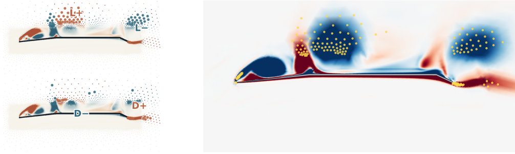
b Geometry (174.1^\circ, 155.0^\circ) , \text{AoA} = 12^\circ
