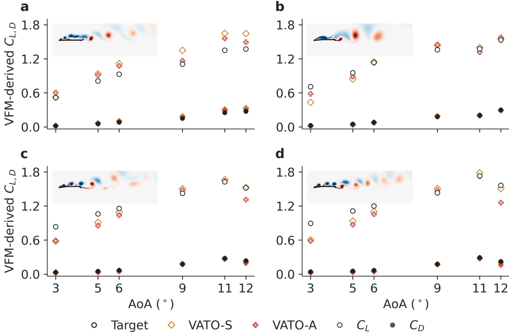
Figure 8: Fixed-geometry VATO predictions of VFM-derived mean C_L and C_D against matched targets. (a–d) The thinnest, median, second-thickest, and thickest geometries of the nine geometry sweep, with (\theta_1, \theta_2) equal to (178.32^\circ, 172.41^\circ) , (174.95^\circ, 158.19^\circ) , (172.46^\circ, 149.04^\circ) , and (171.63^\circ, 146.31^\circ) . Within each geometry and AoA, each point is the mean force coefficient over all direct predictions at lead times 1–30 ms. Circles are the target values; diamonds and crosses are the mean force coefficients predicted by VATO-S and VATO-A. Open markers denote C_L and filled markers denote C_D . The overlay in each panel shows a target-vorticity snapshot at AoA = 12^\circ for the same geometry, rendered on the native mesh with the common w \in [-1000, 1000] \text{ s}^{-1} range.
