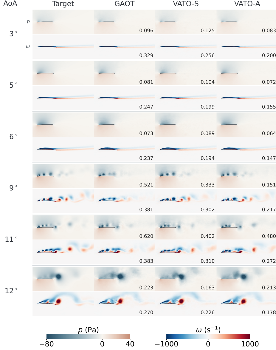
Figure 11: Predictions by the three models for the same geometry, (\theta_1, \theta_2) = (176.6^\circ, 165.1^\circ) , at a lead time of 20 ms. Rows span the six test incidences; columns compare the target with the three predictions. Each cell places the pressure field above the vorticity field, and the numbers on the prediction tiles give the unclipped relative L_2 error over the valid fluid points. All panels share x/c \in [-0.30, 3.50] and y/c \in [-0.73, 0.77] , with colour ranges p \in [-80, 40] Pa and \omega \in [-1000, 1000] s^{-1} .
