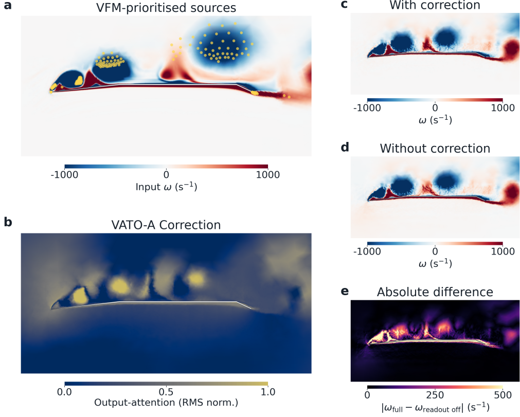
Figure 9: Output-level residual cross-attention correction in VATO-A for one input from the test population, with the geometry, AoA, source time, and lead time fixed in advance. The geometry is (\theta_1, \theta_2) = (174.1^\circ, 155.0^\circ) at \text{AoA} = 12^\circ , with source time 0.081 s and lead time \tau = 10 ms. (a) Current-input vorticity w with the realised VFM-prioritised source locations at the trained budget of 256 tokens; the spatial-coverage locations are omitted from the display. (b) RMS magnitude of the output-level residual correction across the normalised [u, v, p] channels, linearly stretched between its fluid-point 5th and 99th percentiles. (c) VATO-A prediction with the output correction. (d) Prediction from the same checkpoint after bypassing only the selected-token global query-readout residual, with the latent residual and the local geometric attention left active. (e) Pointwise absolute vorticity difference between (c) and (d). Vorticity panels use [-1000, 1000] \text{ s}^{-1} and the difference panel [0, 500] \text{ s}^{-1} ; clipping affects the display only.
