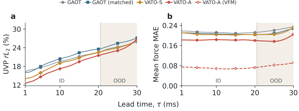
Figure 6: Lead-time-resolved absolute errors on the 54-trajectory population. At each lead time, errors are averaged over the 28 anchors within each trajectory, over the six evaluated incidences within each geometry, and then with equal weight over the nine geometries. (a) Equal-channel UVP relative L_2 error for GAOT, GAOT (matched), VATO-S, and VATO-A. (b) Equal mean of pressure-derived C_L and C_D MAE at each lead time for all four configurations, with the VFM-derived VATO-A result shown as an additional dashed curve. In-distribution (ID) training range ( \tau = 1 –20 ms) and the temporal extrapolation beyond the maximum training lead-time, out-of-distribution (OOD) range ( \tau = 21 –30 ms).
