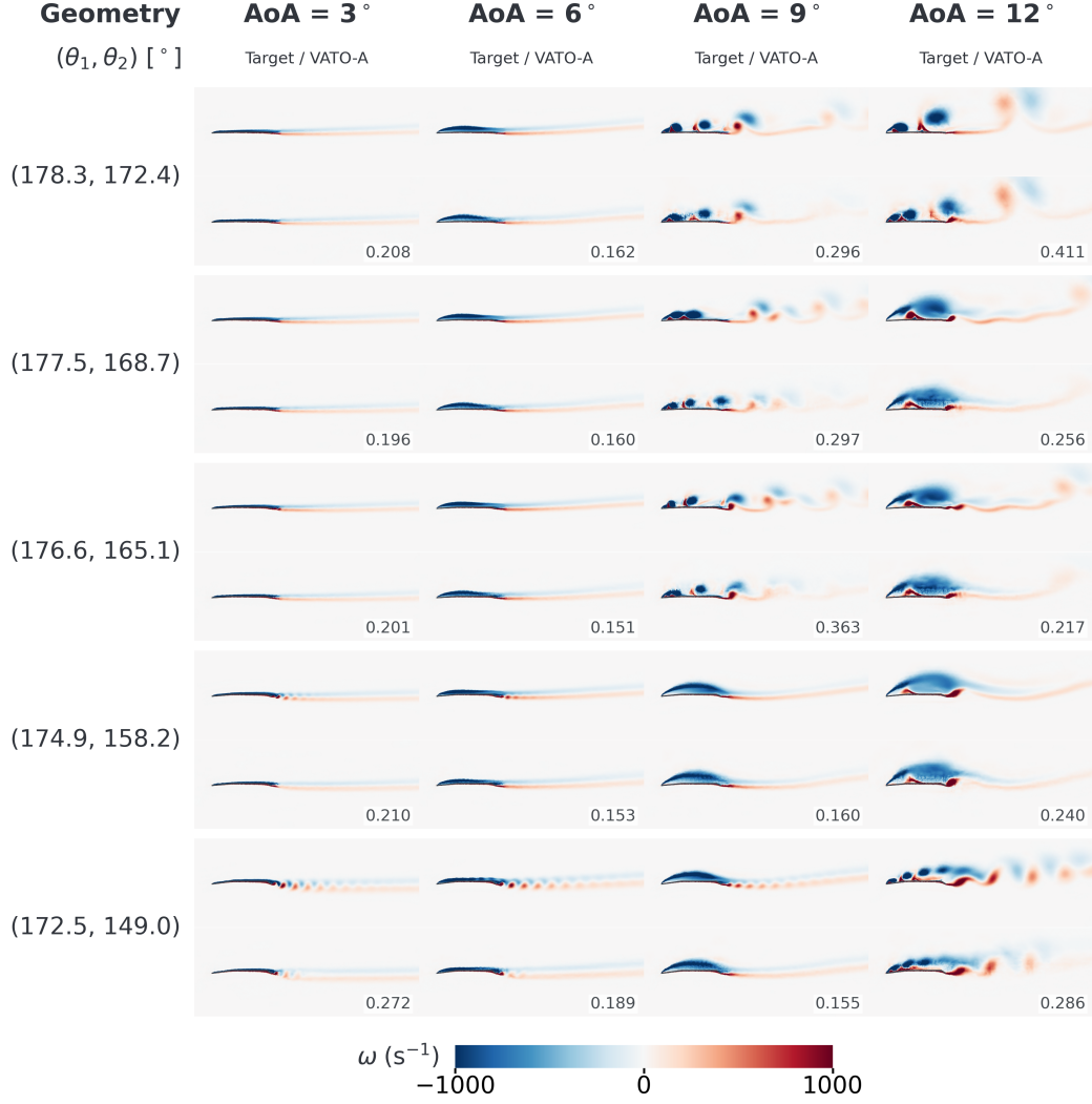
Figure 12: VATO-A predictions of the vorticity field across geometry and incidence at a lead time of 20 ms. Rows show five randomly selected test geometries indexed by the interior fold angles ( \theta_1, \theta_2 ); columns show four incidences. Each cell places the target vorticity above the VATO-A prediction, and the number on each prediction gives the unclipped relative L_2 error over the valid fluid points. All panels share x/c \in [-0.30, 3.50] , y/c \in [-0.73, 0.77] , and w \in [-1000, 1000] s -1 .
