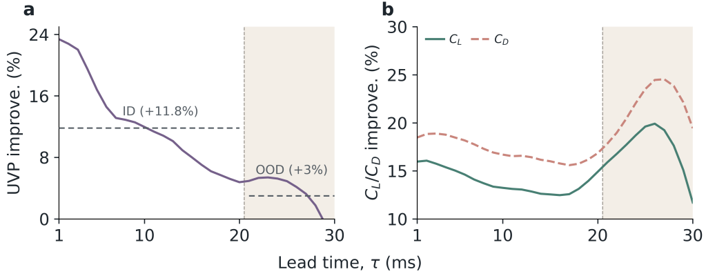
Figure 7: Lead-time-resolved improvement of VATO-A over the GAOT reference on the same reported 54-trajectory population. (a) Equal-channel UVP relative L_2 improvement. (b) Pressure-derived C_L and C_D MAE improvement. Improvement is defined as 100(E_{\text{GAOT}} - E_{\text{VATO-A}})/E_{\text{GAOT}} , where E denotes UVP relative L_2 error in (a) and the corresponding C_L or C_D MAE in (b); positive values favour VATO-A. The dashed horizontal segments in (a) report window-level improvement after averaging each model’s error over the ID and OOD.
