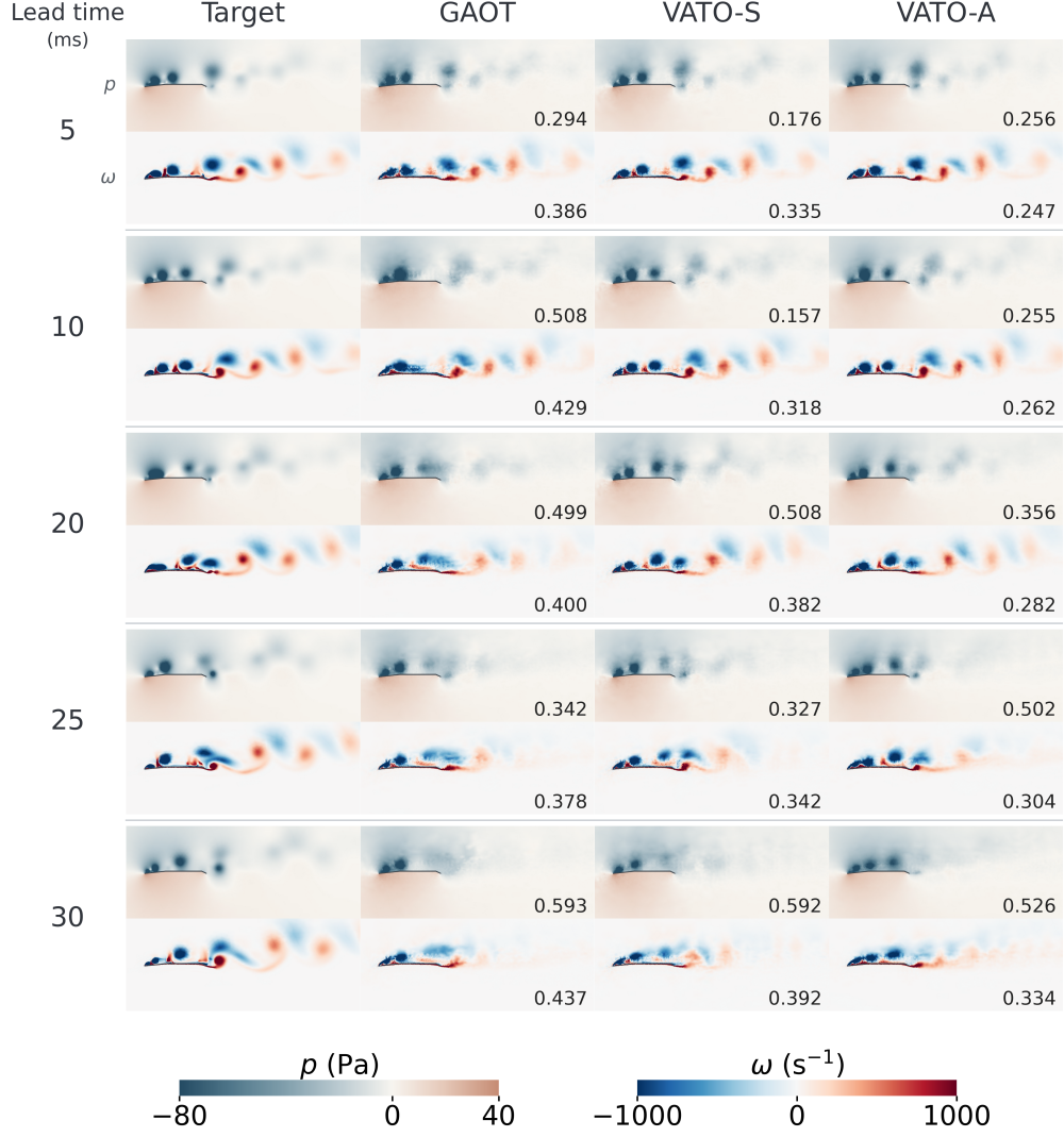
Figure 10: Predictions of the pressure and vorticity fields by the three models for the same case, (\theta_1, \theta_2) = (174.1^\circ, 155.0^\circ) at AoA = 12^\circ , with a source time of 0.081 s. Rows show lead times of 5, 10, 20, 25, and 30 ms; columns compare the target with the three predictions. Each cell places the pressure field above the vorticity field, and the numbers on the prediction tiles give the unclipped relative L_2 error over the valid fluid points. All panels use x/c \in [-0.30, 3.50] and y/c \in [-0.73, 0.77] , with colour ranges p \in [-80, 40] Pa and w \in [-1000, 1000] s^{-1} .
