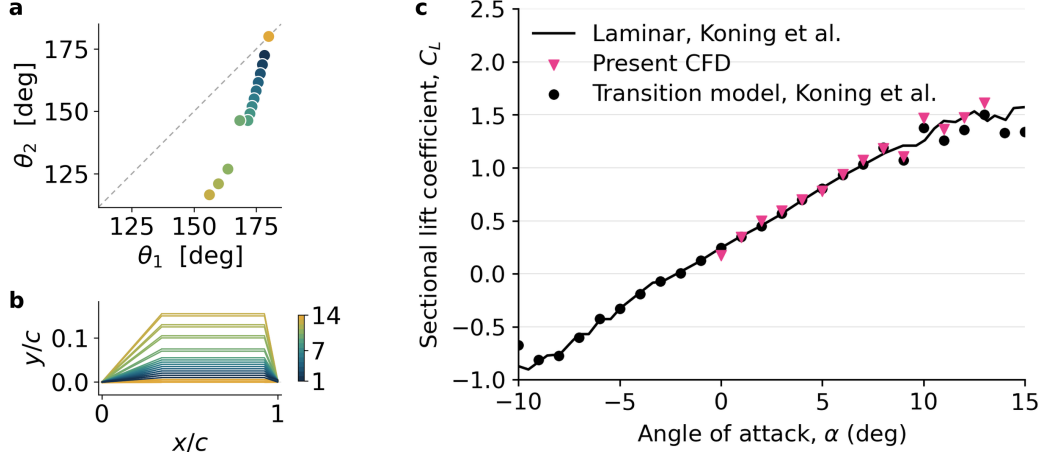
Figure 1: Dataset geometry and CFD cross-check. (a) Envelope in (\theta_1, \theta_2) interior-fold-angle space; the dashed diagonal denotes \theta_1 = \theta_2 . (b) Chord-normalised surface contours of the fourteen DEP geometries, coloured by geometry index. (c) Time-averaged sectional C_L from the present STAR-CCM+ simulations, compared with the transition-model and fully laminar results computed by Koning et al. [32] on the matched configuration.
