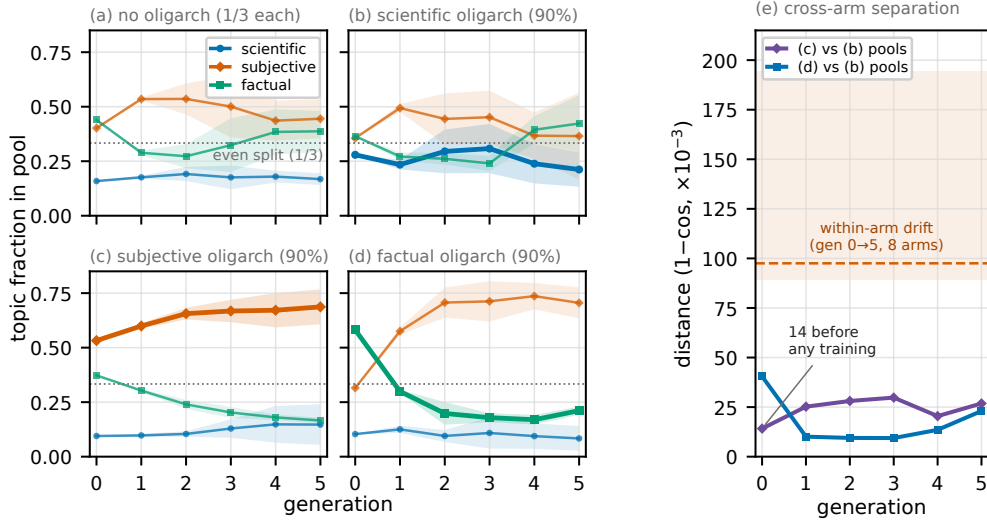
Figure 2: The K=3 injected probe. (a)–(d): topic composition of the mixed pool by generation; the bold curve is the topic injected into that panel’s oligarch ((a) has no oligarch); shading is \pm 1 s.d. over 3 seeds; absolute heights are not comparable across panels (Appendix B). (e): distances from the pool centroids of arms (c) and (d) to that of (b); the band is the min–max range of five-generation drift over the eight probe arms, the dashed line their median (three high arms pull it off center).
