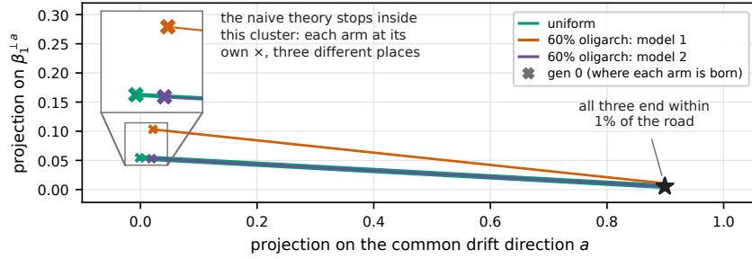
Figure 8: The toy model of Appendix E: three arms (uniform, two different oligarchs), common-drift fraction 0.9. Horizontal axis: projection onto the common direction a ; vertical axis: one dimension perpendicular to it; plotted is each arm’s share-weighted mean of model positions (the pool). The inset magnifies the departure cluster 2.4\times (a length ratio); the \times marks are where each arm would end under zero common drift. The cluster’s width, 7.5% of the full journey, is the one quantity set from data (inverting generation-0 separation 0.0333 against five-generation drift 0.4438, in distance units); the fraction 0.9, the number of models, and the directions are arbitrary. Axes to scale; no generation ticks—the toy’s clock does not align with the observed generations; toy units are not comparable to the text’s \times 10^{-3} distances.
