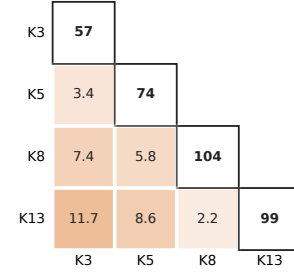
Figure 4: Generation-5 geometry of the four nested ecosystems, each represented by its 28% Phi-2 arm. Diagonal: each ecosystem’s own generation-0-to-5 drift; off-diagonal: distance between two ecosystems at generation 5, darker meaning farther ( 1 - \cos , \times 10^{-3} ).
