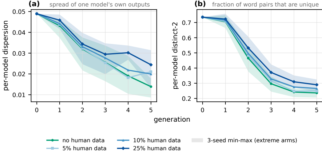
Figure 7: The uniform arm of the K=3 injected probe, with four doses of human text in the shared pool (0%, 5%, 10%, 25%). Both panels measure each model’s own newly generated text, not the mixed pool—the pool is diluted by the injected human lines, and measuring it would hand the remedy a free win. (a) Internal dispersion of one model’s output batch, defined as 1 minus the mean cosine of each text to that model’s centroid, encoded by the main text’s frozen DeBERTa. (b) distinct-2 of the same batches, passing through no encoder. Curves are 3-seed means; shading is the 3-seed min–max range, drawn only for the two extreme arms (0% and 25%)—with n=3 , four bands would paint precision the seeds cannot support. The four arms coincide at generation 0 by construction: these quantities read each model’s own output, and generation-0 models are not yet differentiated by arm. Vertical axes are raw values, not the text’s \times 10^{-3} distances, and the two panels are not comparable. A third reading (cross-model distance) was computed and not plotted; the reason is in the section text.
