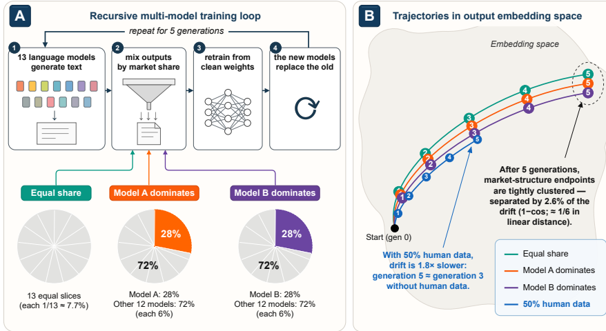
Figure 1: Experimental setup and result preview. (A) One generation of the ecosystem loop, iterated five times; the bottom row shows three example market-share settings. (B) Schematic trajectories, in output embedding space, of the centroid of each arm’s model-generated pool text (human-data arms embed only the model-output portion, matching Section 3): trajectory positions are illustrative; the annotated 2.6% (in 1 - \cos ; roughly 1/6 in linear distance) and 1.8\times are measured values from Section 4.
