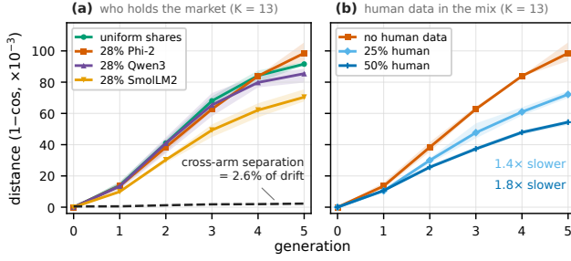
Figure 3: Two knobs in natural ecosystems: (a) the four share arms of K=13 ; (b) the oligarch arm of K=13 at human-data doses of 0%, 25%, and 50%, all sharing generation 0. Vertical axis: each arm’s distance from its own generation 0 ( 1 - \cos , \times 10^{-3} ); shading: 3-seed min-max; dashed line in (a): mean between-arm separation per generation. The text’s on-path statements are two-point distances, not differences of heights here.
