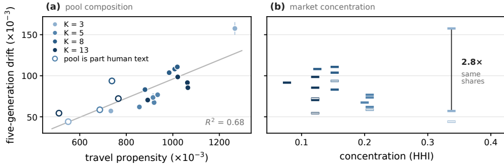
Figure 5: Five-generation drift of the nineteen arms against pool composition (a) and concentration (b); hollow marks: pools that are part human text. Error bars in (a): s.e. of the 3-seed mean; the line is a least-squares fit to all nineteen arms. In (b) each arm is a bar at its HHI; the arms share only seven values.
