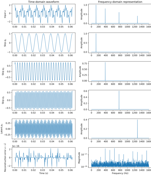
Fig. 2. Single-channel residual routing of four orthogonal sinusoidal factors. q_1, q_2, q_3 isolate three components while p_3 retains the fourth; their sum reconstructs the input.
