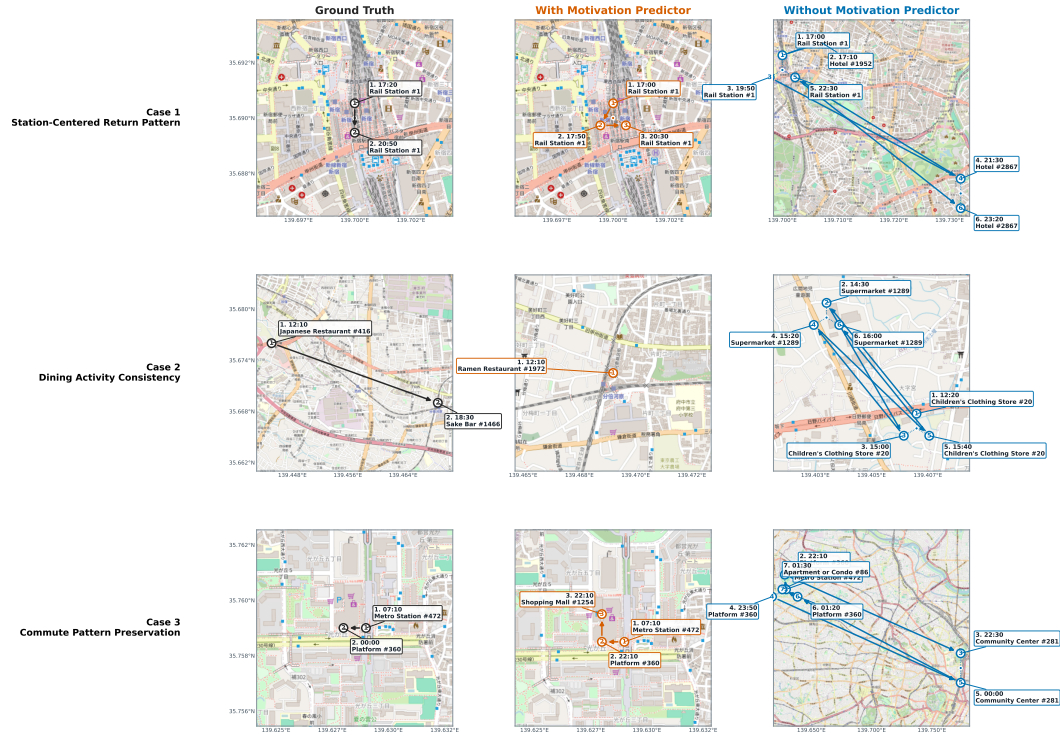
Figure 4: Trajectory comparisons with and without the trained motivation predictor. From left to right, the columns show the ground-truth trajectory, MotiveMob with the motivation predictor, and the corresponding ablation without it. Numbered markers indicate visit order, and labels show the visit time and POI.
