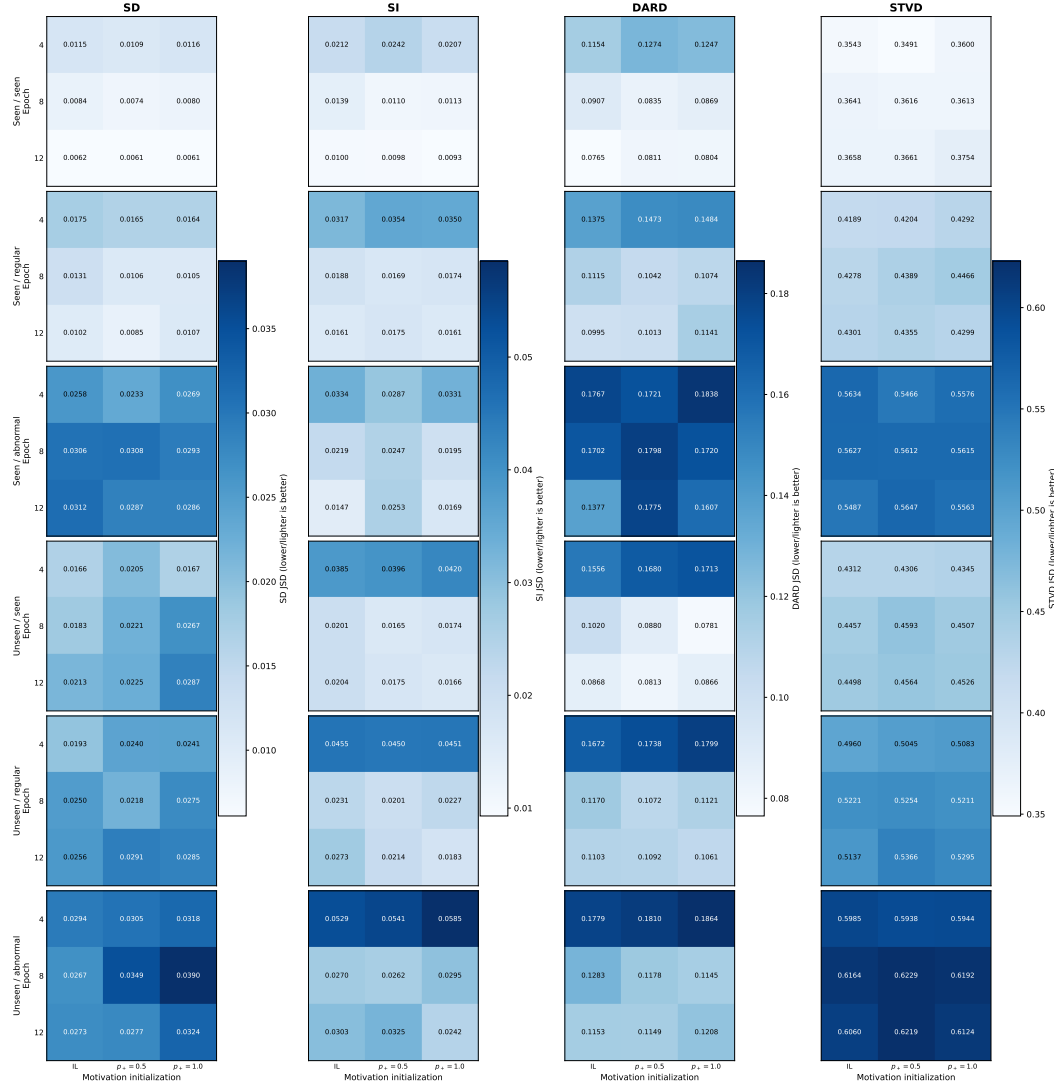
Figure 5: Motivation-predictor sensitivity to IWM initialization and training duration. Each evaluation split contains four 3 \times 3 matrices corresponding to SD, SI, DARD, and STVD. Rows show results after 4, 8, and 12 epochs of motivation-predictor training, while columns show direct IL, balanced IWM initialization ( p_+ = 0.5 ), and observed-only IWM initialization ( p_+ = 1.0 ). Cell annotations report raw JSD values; lower values and lighter shading indicate better distributional alignment.
