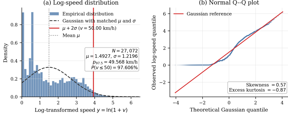
Figure 3: Distributional diagnostics for the log-transformed transition speeds used to calibrate v_{\max} . (a) Empirical distribution and a Gaussian distribution with the same mean and standard deviation. The red line marks the two-standard-deviation upper bound. (b) Normal Q–Q plot showing the remaining deviations from Gaussianity, particularly in the tails.
