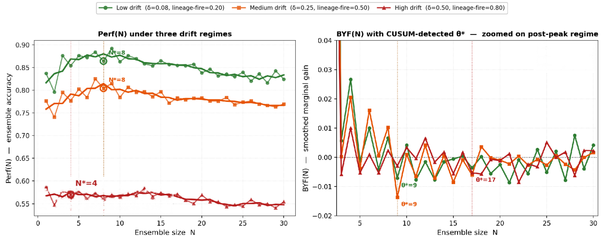
Figure 4. Simulation-based validation of the UoU framework. Left: ensemble performance \text{Perf}(N) across three drift regimes, with N^* marked. Right: smoothed \text{BYF}(N) with CUSUM-detected \theta^* (zoomed on the post-peak regime to make the crossings visible).
