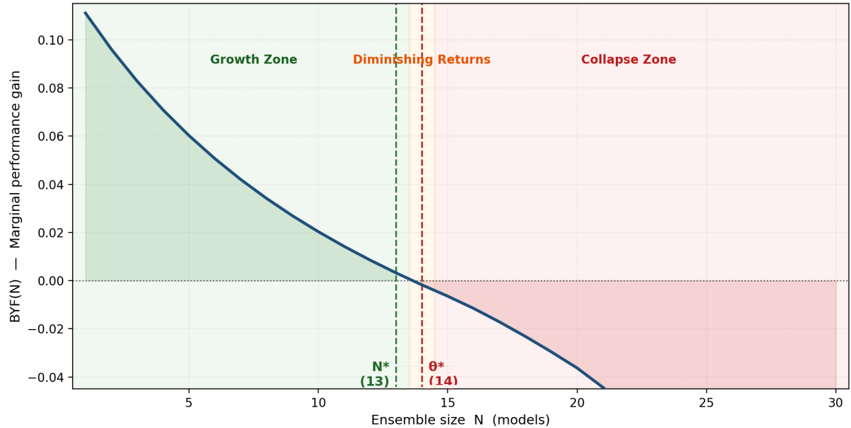
Figure 2. Conceptual BYF curve with three ensemble-size regimes. Growth Zone ( N < N^* ): each additional model contributes positive marginal gain. Diminishing Returns Zone ( N^* \leq N < \theta^* ): BYF is positive but declining. Collapse Zone ( N \geq \theta^* ): BYF is negative: adding models actively degrades ensemble performance.
