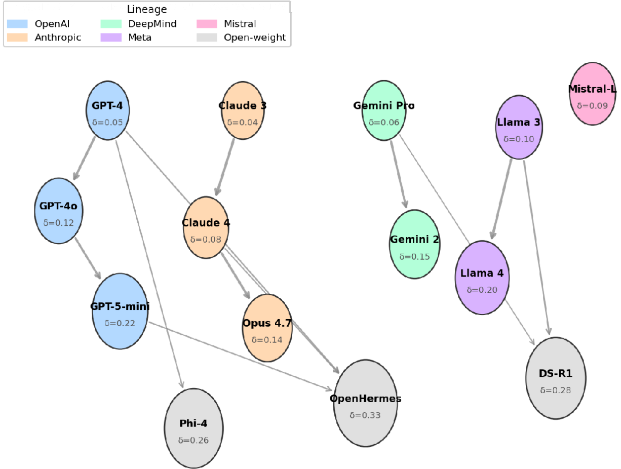
Figure 1. Illustrative Universe Graph (subset of ~14 models across 6 lineages). Node size is proportional to the EHD drift coefficient \delta_m ; arrow thickness to the training-data contamination weight w_{ab} . Within-lineage edges (bold) and cross-lineage edges (thin) both contribute to aggregate ensemble drift.
