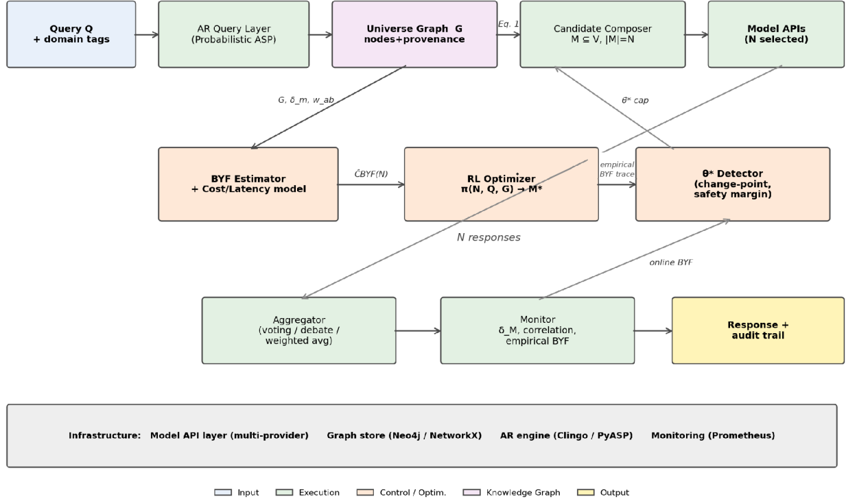
Figure 3. UoU reference architecture. The top pipeline handles query ingress, AR-driven ensemble composition from the Universe Graph, and model-API invocation. The middle band contains the BYF estimator, RL ensemble optimizer, and \theta^* detector. The bottom band contains the aggregator and the monitoring component that feeds empirical BYF back into \theta^* detection, closing the control loop.
