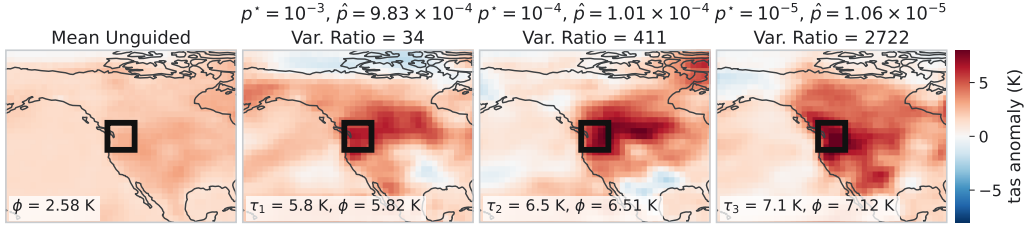
Figure 3: Surface-temperature anomaly (K) for July at \Delta T = +1.5 K over the Pacific Northwest (PNW) target region. Left : average \text{tas} field over 10^7 samples. Remaining panels : the highest-weight crossing particle produced by the guided sampler at different exceedance thresholds \tau and regional average temperature \phi(\cdot) of the sample. p^* are MC estimates; \hat{p} is obtained from the guided estimator; full results in Table 15. The variance ratio (Var. Ratio) at matched compute is defined as \text{Var}(\hat{p}_{\text{unguided}})/\text{Var}(\hat{p}_{\text{guided}}) .
