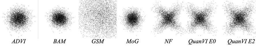
Figure 5: Sample visualization on the first two dimensions of the X-shape target with D = 20 , comparing all baselines with our method.
