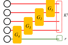
(b) A simple QTN example. TNs represent high-dimensional tensors through contractions of low-order core tensors connected by a sparse graph structure. A QTN is a circuit-like TN architecture with additional unitary constraints on local core tensors. In this figure, circles denote open indices with local dimension K , while rectangles denote order-4 core tensors with dimensions K \times K \times K \times K . The red lines represent system wires, and the green lines represent auxiliary wires for mixed-state representations, which will be introduced in Section 4.2.2.
