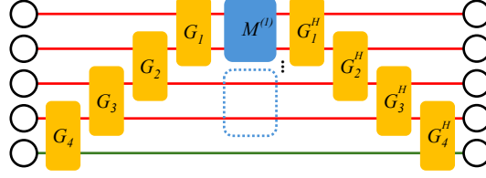
Figure 2: Graphical representation of a local training contraction. The yellow tensors form the QTN representation of U_\Theta and U_\Theta^\dagger , while the blue tensor denotes a local score-based loss operator M^{(d)} . Red wires denote system wires and green wires denote ancilla wires. Open circles denote fixed boundary vectors used to close the finite QTN contraction.
