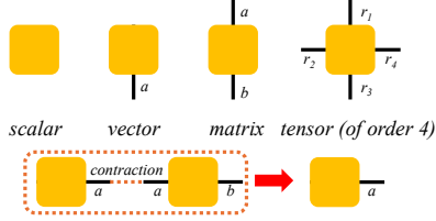
(a) Graphical notation of tensors and tensor contraction. Each node represents a tensor, and each edge represents an index (mode) of the tensor. The label on an edge indicates the dimension of the corresponding mode. For example, a vector has one index with dimension a , a matrix has two indices with dimensions a \times b , and an order-4 tensor has four indices with dimensions r_1 \times r_2 \times r_3 \times r_4 . When two tensors are connected by an edge, they share the same index. The operation of contracting this edge, called tensor contraction, corresponds to summing over the shared index.
