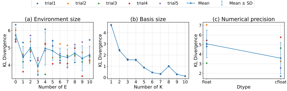
Figure 3: Ablation studies of QuanVI.
