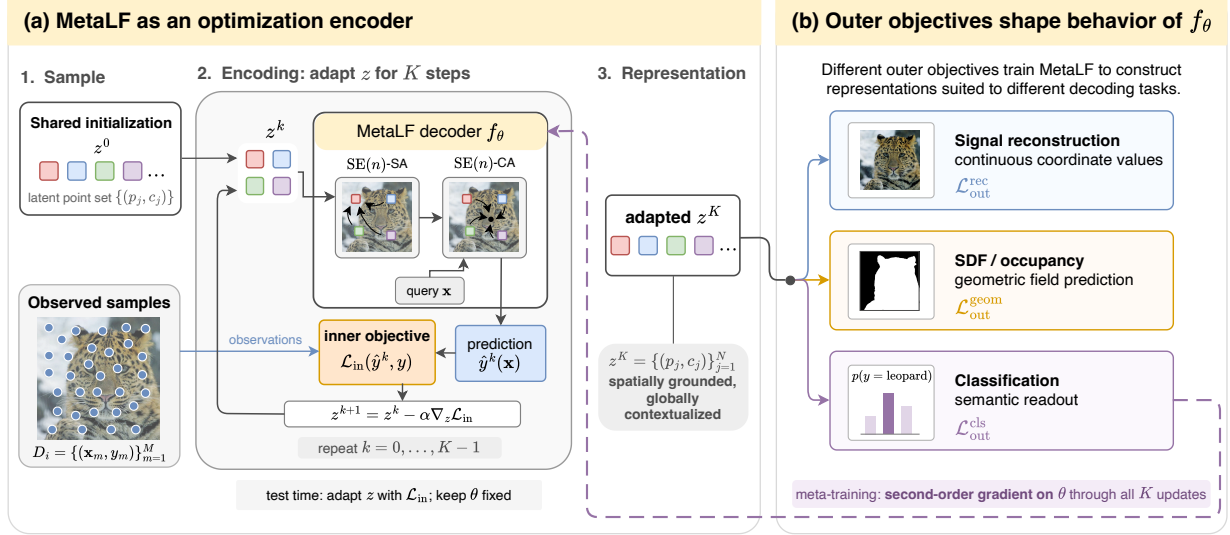
Figure 3: MetaLF as an optimization encoder. (a) K gradient updates encode observations into a spatially grounded, globally contextualized latent representation through \text{SE}(n) -equivariant self-attention (SA) layers and cross-attention (CA) with a query coordinate. (b) During meta-training, task-specific outer objectives can shape the decoder through second-order gradients across the adaptation steps. Global contextualization of the latent point set therefore enables flexible meta-training: the same inner-loop encoder can learn representations tailored to diverse downstream objectives.
