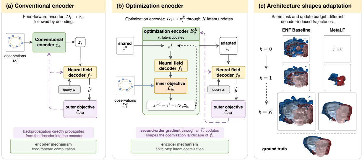
Figure 2: Second-order meta-learning trains an optimization encoder whose behaviour is shaped by decoder architecture. (a) A conventional encoder maps an observed signal to a latent representation z_i , which the decoder evaluates at a query coordinate \mathbf{x} . (b) In meta-learned neural fields, an explicit encoder is replaced by K gradient updates on z , forming an optimization encoder. Second-order differentiation propagates the outer objective \mathcal{L}_{\text{out}} through these unrolled updates, jointly shaping the finite-step encoding behavior and the decoder f_\theta . (c) Because the decoder induces the latent updates, its architecture shapes the resulting adaptation trajectory. ENF represents a local fitting model, lacking direct exchange of context among localized latents. MetaLF instead coordinates these latents through attention. This shared context produces coherent updates that quickly capture non-local structure, as illustrated by fitting cardiac signed distance functions.
