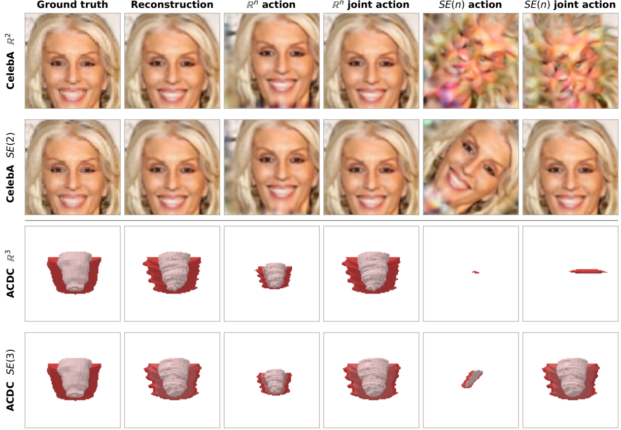
Figure 5: MetaLF is equivariant under a group action defined by its bi-invariant feature a . Rows show translation-equivariant ( \mathbb{R}^n ) and roto-translation-equivariant ( SE(n) ) MetaLF models on CelebA and ACDC myocardium. Columns show ground truth, reconstruction in the canonical frame, pose-only translation, joint translation of poses and queries, pose-only roto-translation, and the corresponding joint roto-translation. Acting on poses alone transforms the represented field; applying the same group element jointly to poses and queries preserves predicted values at corresponding coordinates when the model respects that symmetry. Accordingly, joint translations match the canonical reconstruction in every row, whereas joint roto-translation does so only for the SE(n) models.
