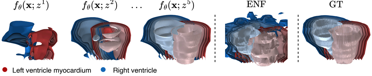
Figure 1: Example use case of MetaLF meta-learning latent cardiac shape representations [3]. The first three panels illustrate smooth shape recovery as a shared latent pointcloud z is refined over k = 1, \dots, 5 gradient steps. MetaLF learns contextualized latent representations that preserve detail while capturing the underlying function, an ill-posed task for local representation models such as ENF [4].
