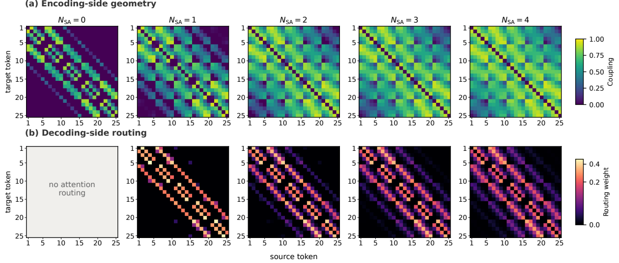
Figure 7: Optimization encoder-side coupling (top) and decoder-side attention routing (bottom) evaluated on the polynomial fields dataset, shown with increasing number of MetaLF self-attention layers ( N_{SA} ) for N = 25 latent tokens. Additional layers allow information to propagate beyond local latent neighborhoods while retaining the spatial structure of the representation.
