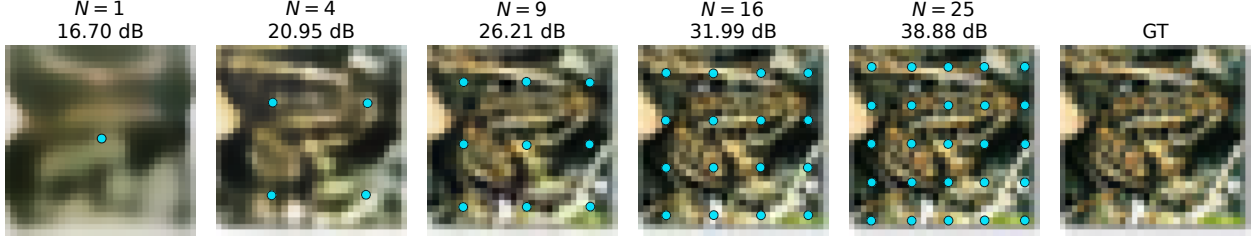
Figure 9: Reconstruction quality as a function of latent pointcloud size. The example uses MetaLF with N_{SA} = 4 and per-latent content size of D = 64 .
