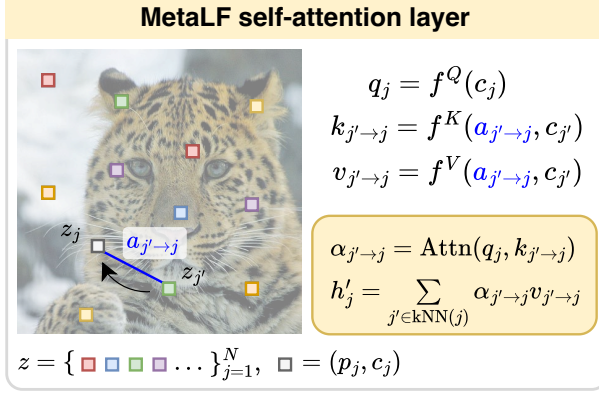
Figure 4: A receiving latent j attends to neighbouring source latents j' using bi-invariant geometric attributes a_{j' \rightarrow j} . Keys and values combine this geometry with the source content c_{j'} , and their attention-weighted aggregation produces the updated feature h'_j .
