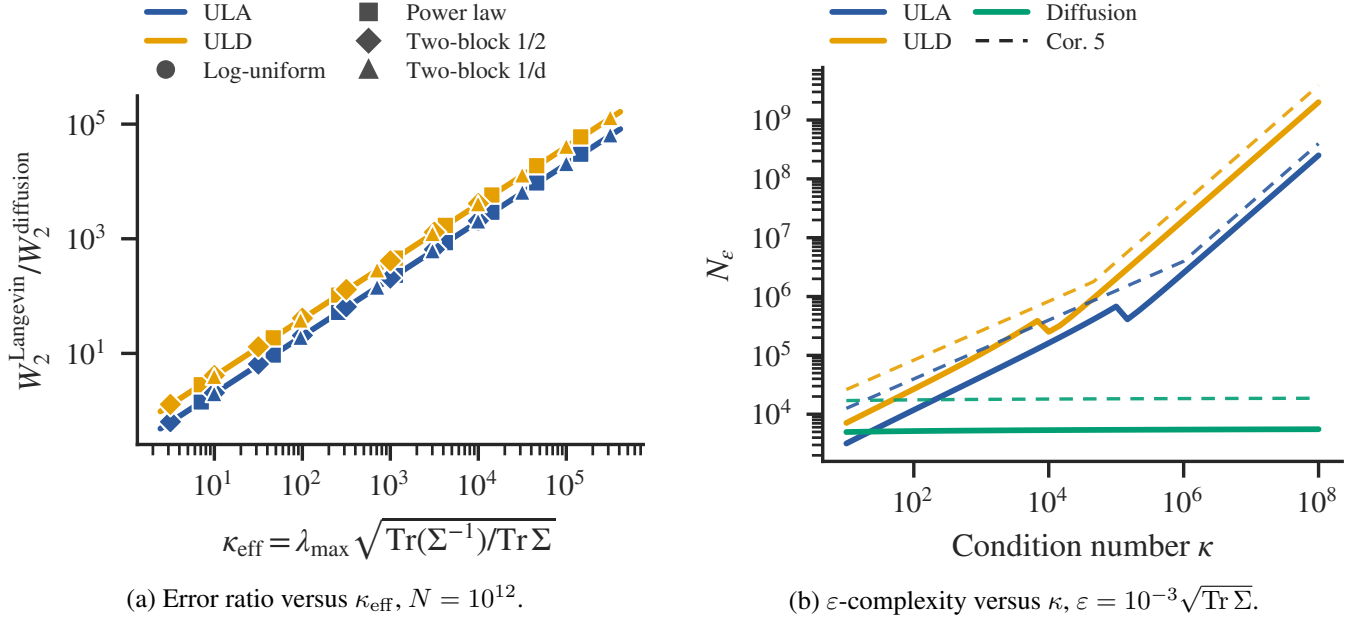
Figure 2: Tightness of the theory in dimension d = 1000 . (a) Ratio W_2^{\text{Langevin}} / W_2^{\text{diffusion}} at budget N = 10^{12} , as a function of \kappa_{\text{eff}} := \lambda_{\text{max}} \sqrt{\text{Tr}(\Sigma^{-1}) / \text{Tr} \Sigma} , for four spectral families with \lambda_{\text{max}} = 1 and \kappa \in \{10, 10^2, \dots, 10^8\} : “log-uniform” ( \lambda_i = \kappa^{-(i-1)/(d-1)} ); “power law” ( \lambda_i = i^{-a} with a = \log \kappa / \log d ); “two-block 1/2” (half of the eigenvalues equal to 1 and half to 1/\kappa ); “two-block 1/d” (one eigenvalue equal to 1 and d - 1 equal to 1/\kappa ). Langevin samplers are tuned as in Theorem 1; the diffusion uses the spectrum-agnostic schedule of Proposition 4 ( T = \sqrt{N} , \delta = 1/N^2 ). Lines are the quotients of the asymptotic equivalents, \frac{1}{5} \kappa_{\text{eff}} (ULA) and \frac{2}{5} \kappa_{\text{eff}} (ULD), with no fitted constant: all four families collapse onto them within 3.4%, consistent with a finite- N correction of order 1/\log N \approx 3.6\% . (b) Budget N_\varepsilon after which the error stays below \varepsilon = 10^{-3} \sqrt{\text{Tr} \Sigma} , where \sqrt{\text{Tr} \Sigma} = W_2(\delta_0, \mathbb{P}) is the scale of the target, for the log-uniform spectrum. Dashed: the sufficient budgets of Corollary 5 ( r = 10 in Remark 6 for the diffusion), within a factor 3 of the observed ones. The diffusion budget does not depend on \kappa . The Langevin budgets follow the \sqrt{\kappa} rate of Table 1 as long as \varepsilon \lesssim \lambda_{\text{min}} \sqrt{\text{Tr}(\Sigma^{-1})} = \sqrt{\text{Tr} \Sigma / \kappa} ; beyond, the burn-in N_\star = \Theta(\kappa \log \kappa) of Remark 2 takes over and the budget grows linearly in \kappa . Kinks on the ULA curve mark the switch between the two branches of its step-size.
