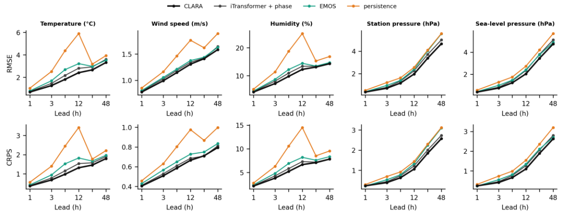
Supplementary Figure 1. Per-variable RMSE (top) and CRPS of the issued distribution (bottom) in physical units by lead for CLARA, iTransformer + phase, EMOS and persistence (96 ASOS, six multi-year folds; RMSE from the fold-mean squared error).
