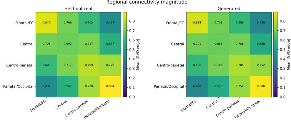
Figure 2: Regional connectivity magnitude on BNCI2014_001. Mean absolute GVD edge magnitude between broad scalp regions for held-out real trials and generated trials. The generated data preserve the relative regional organization of the real EEG, including strong within-region Frontal/FC and Parietal/Occipital connectivity, strong Central–Centro-parietal coupling, and weaker long-range Frontal/FC–Parietal/Occipital interactions.
