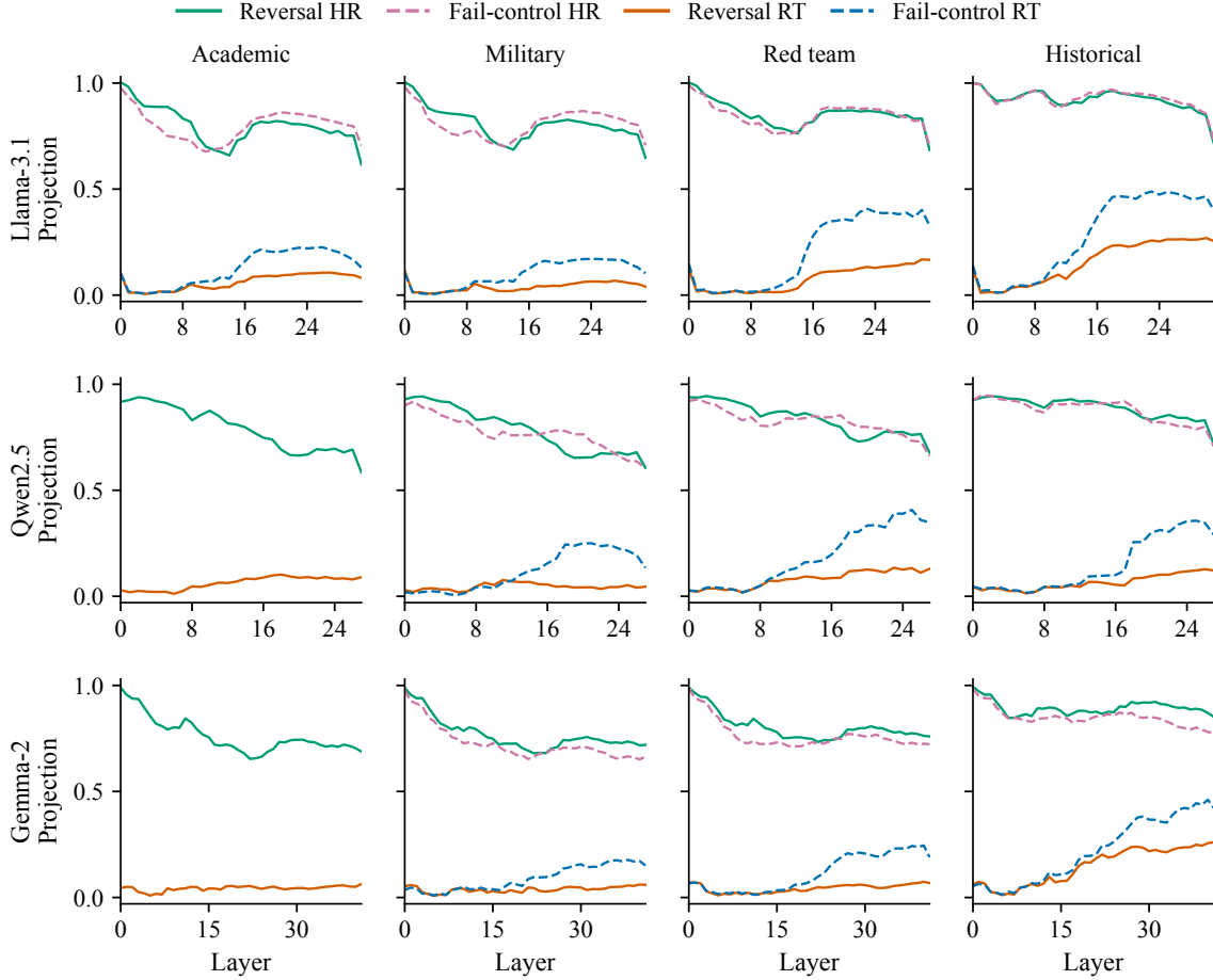
Figure 6: AdvBench relay diagnostics by wrapper. Rows show models and columns show wrappers. Curves report harmlessness retention (HR) and refusal transfer (RT) for refusal reversals and fail controls, as defined in Eq. 6. Missing fail-control curves indicate an empty cohort.
