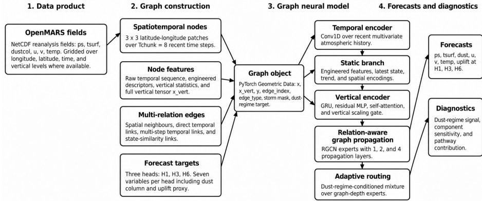
Fig. 1 Overview of the MaGMA workflow. OpenMARS gridded atmospheric fields are transformed into graph-structured learning objects by partitioning the data into local spatiotemporal patches, constructing node features from recent temporal history, engineered descriptors, and vertical column information, and connecting nodes through spatial, temporal, multi-step temporal, and atmospheric-state similarity edges. During graph construction, each node is also assigned multi-horizon targets corresponding to H1, H3, and H6. The resulting graph object is processed by a neural forecasting architecture that combines temporal encoding, static and engineered features, vertical column encoding, relation-aware graph propagation, adaptive routing, and horizon-specific residual forecast heads. The model predicts surface pressure, surface temperature, dust column, zonal wind, meridional wind, atmospheric temperature, and uplift at each horizon.
