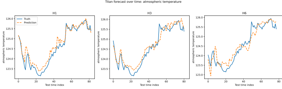
Fig. 5 Supplementary Titan forecast demonstration showing truth and predicted temporal evolution for atmospheric temperature across the H1, H3, and H6 forecast heads. Each panel has the spatial mean over the Titan test graph at each test time step. This figure is included as a cross-planet portability demonstration of the graph-construction and multi-horizon forecasting framework rather than as a full Titan atmospheric forecasting study.
