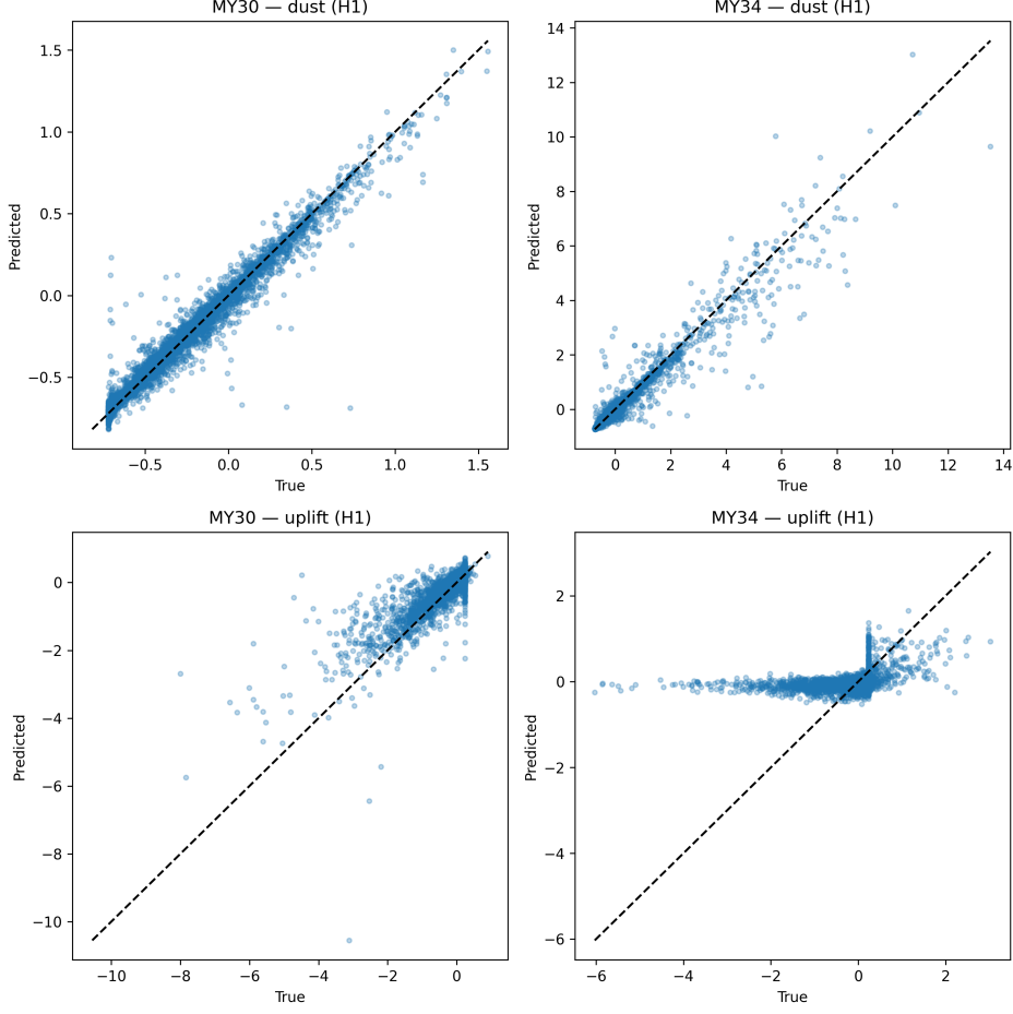
Fig. 2 Truth-versus-prediction scatter plots for MY30 and MY34 at H1, comparing dust-column and uplift forecasts. Dust-column predictions remain closely aligned with the one-to-one reference line, while uplift predictions show weaker agreement, particularly under the MY34 global dust storm regime.
