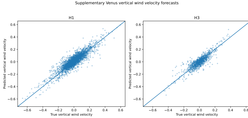
Fig. 4 Supplementary Venus truth-versus-prediction forecasts for vertical wind velocity at H1 and H3. The plotted field corresponds to vitw in the Venus dataset. This figure is included as an ability demonstration showing that the graph construction and multi-horizon forecasting pipeline can be used on a non-Martian planetary atmospheric dataset.
