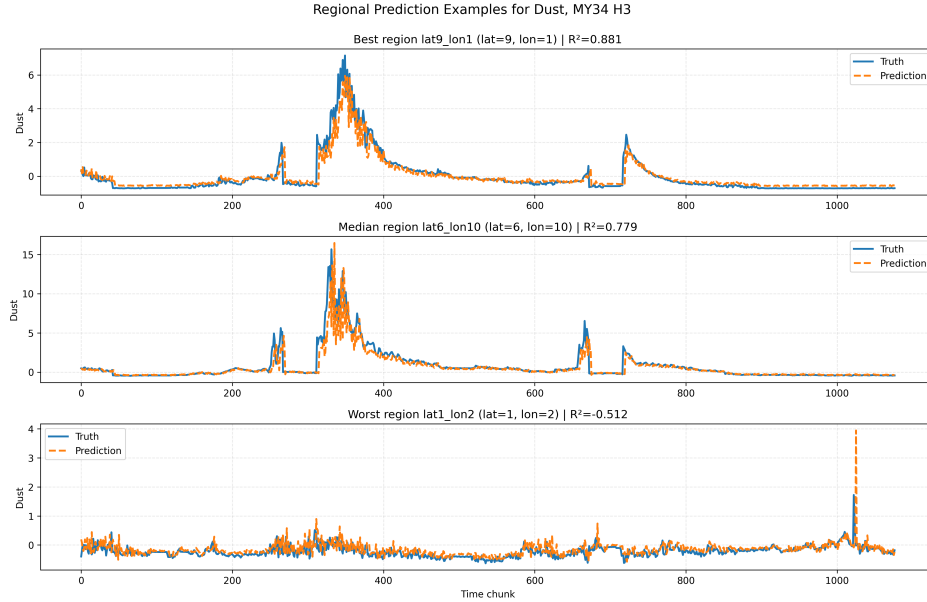
Fig. 3 Regional prediction examples for MY34 dust-column forecasting at H3. The panels show representative best-case, median-case, and worst-case spatial regions. The best and median regions demonstrate that the model can track the main dust evolution in some locations, while the worst-case region illustrates a regional failure mode with a false positive late spike.
