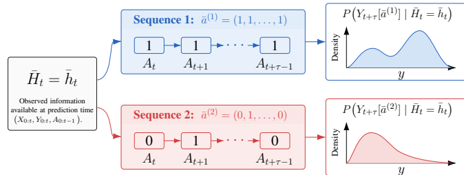
Figure 1: Task: Estimating the CDPOs under different treatment sequences.
