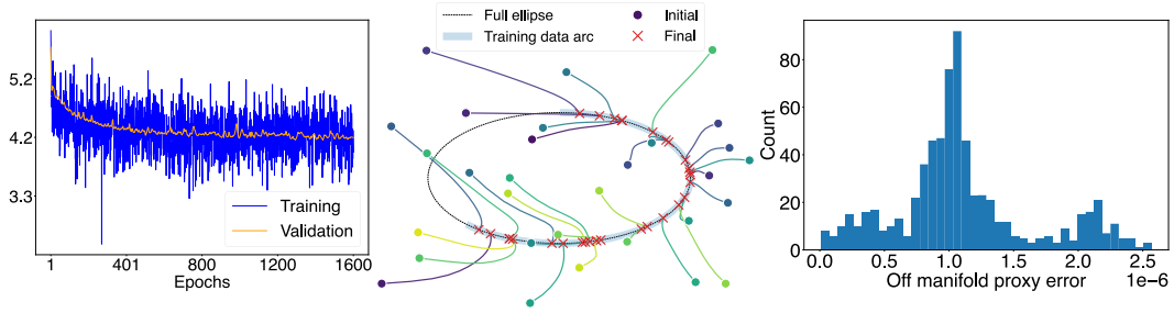
Figure 2: Ellipse: training/validation losses over 1,600 epochs, sampling trajectories, and terminal off-proxy errors for 700 samples. Here, we approximate the manifold (the ellipse) by local affine proxies using PCA.
