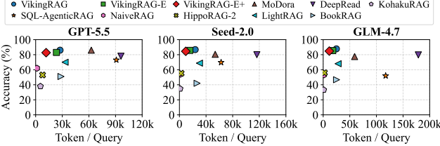
Figure 7: Variation of Backbone LLMs on VersionQA.
