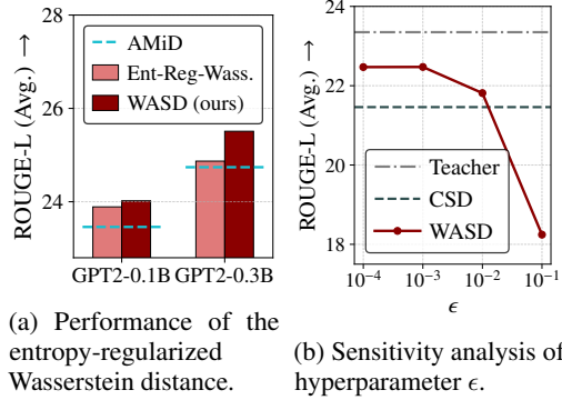
Figure 4: Ablation studies of WASD.
