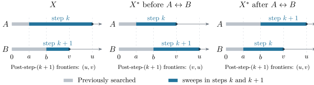
Figure 2: Comparison of X and X^* in Lemma 2. After relabelling, the frontiers of X^* match those of X , allowing the same continuation of the algorithm.
