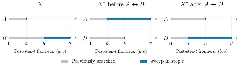
Figure 1: Comparison of X and X^* in the proof of Proposition 1.
