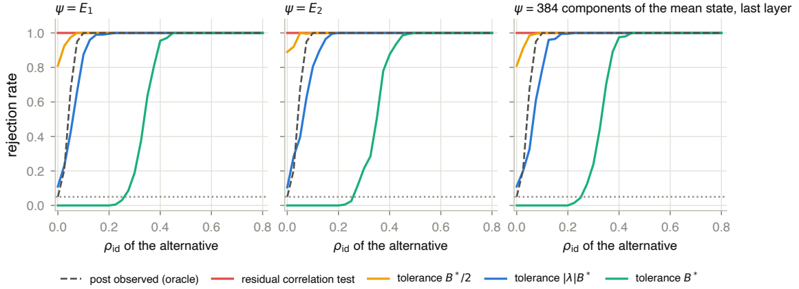
Figure D.7: Experiment 3, rejection rates against the coupled alternatives for \psi = E_1, E_2 and 384 principal components of the generator’s mean state at the last layer, by the conditional correlation \rho_{\text{id}} of comment and summary given the post, over 200 datasets per value: the residual correlation test, the robust test with the tolerance equal to half the true insufficiency, to the true bias and to the true insufficiency ( B^* in the legend), and the reference test that conditions on the post through the unused draws ( Appendix C.7 ).
