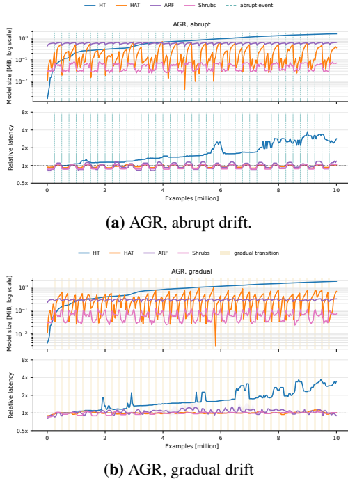
Figure 6: Model size and prediction-plus-update latency. Teal dashed lines mark abrupt events, and pale-gold intervals mark gradual transitions.
