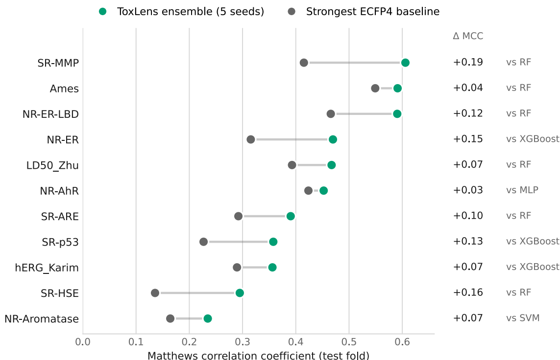
Figure 2: Per-endpoint held-out test MCC for the five-seed ToxLens ensemble and the strongest ECFP4 shallow baseline. For each endpoint, the strongest shallow comparator is selected from Random Forest, XGBoost, multilayer perceptron, and support-vector machine. Every model used the same split and a threshold selected on its own validation probabilities. The plot is descriptive: ToxLens achieved the highest MCC for all 11 endpoints, while the identity of the strongest shallow comparator varied by endpoint. Complete values for all models are reported in Supplementary Table 2.
