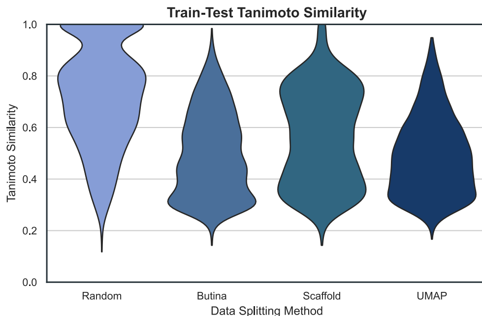
Supplementary Figure 1: Train-test Tanimoto-similarity distributions for Random, Butina, Bemis-Murcko scaffold, and UMAP-HDBSCAN partitions. For each test molecule, similarity is measured against its nearest training-set neighbour; lower distributions indicate stronger structural separation. Complementary scaffold-novelty, property-balance, and aggregate out-of-distribution statistics are reported in Supplementary Table 3.
