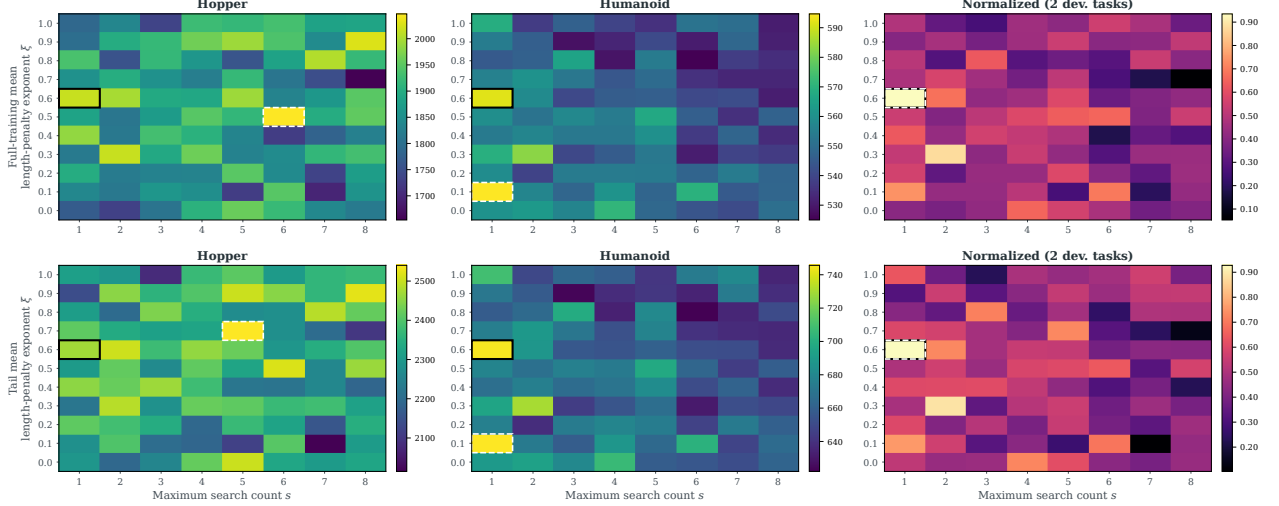
Figure H.1: \xi \times s grid on the MuJoCo development tasks. Top: full-training mean return; bottom: tail return. Black outline: the selected configuration (0.6, 1) ; white dashed outline: the best cell of each panel. The right-most column averages the min-max-normalized grids of Hopper-v4 and Humanoid-v4.
