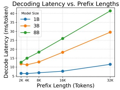
(b) Single token decode latency across prefix lengths and model sizes.
