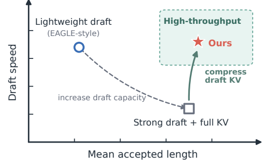
Figure 1: Lightweight drafts are fast but accept fewer tokens; strong full-KV drafts recover acceptance but incur high KV-access cost. Our compressed-memory draft targets high acceptance and speed.
