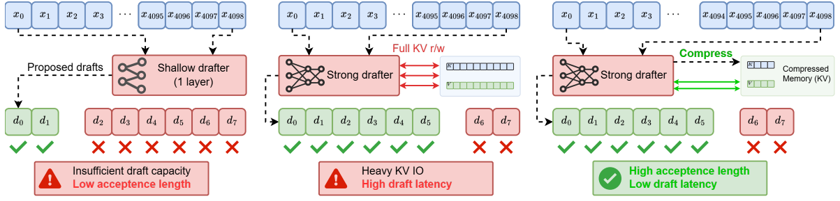
Figure 2: Overview of our proposed framework.
