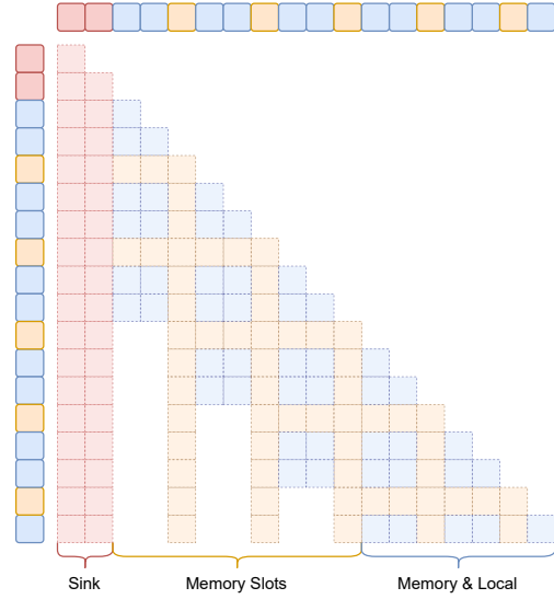
Figure 7: Memory prefill attention mask.
