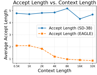
(a) Accepted draft length of EAGLE compared with the 3B draft model for Llama3.1-8B. Both methods use a 10 as draft length.
