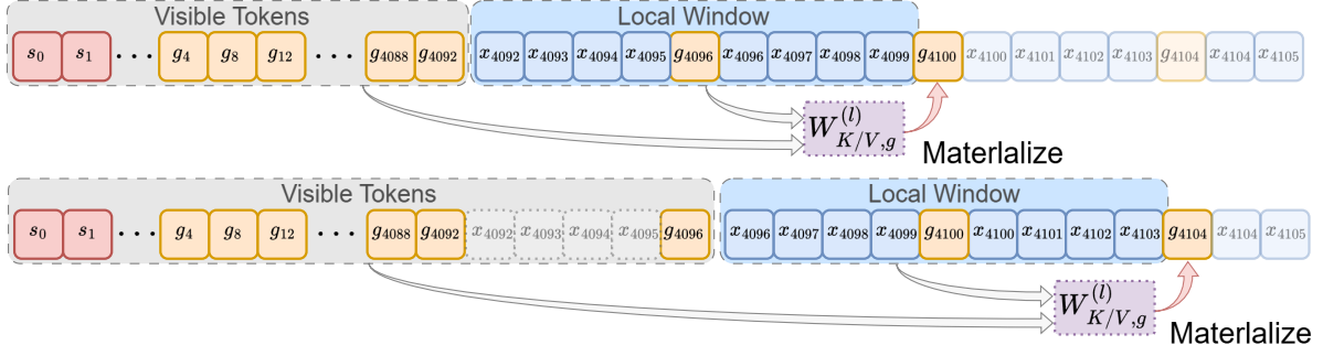
Figure 4: Memory-augmented sliding-window drafting at two consecutive compression boundaries. Top: the draft materializes slot g_{4100} at the current boundary. Bottom: the window has advanced by one slot interval (after 4 decoding steps); the oldest raw KV is evicted, the previously materialized slot is retained as memory, and the next slot g_{4104} is produced at the new boundary.
