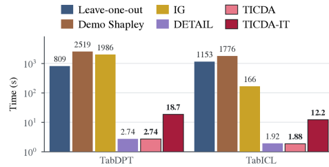
Figure 2: Average computation time per method.
