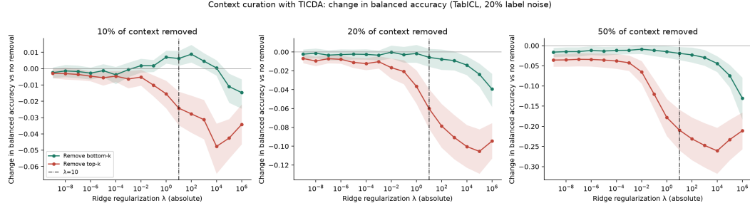
(a) Context curation sensitivity to \lambda .
