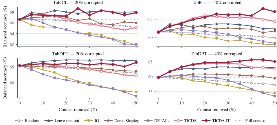
Figure 3: Curation: aggregated balanced accuracy evolution on TabDPT and TabICL under different levels of demonstration corruption. Each method ranks in-context demonstrations by its attribution scores, and the lowest-scored demonstrations are removed.
