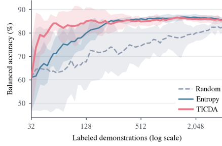
Figure 4: Balanced accuracy evolution on APSFailure against the number of labeled demonstrations.
