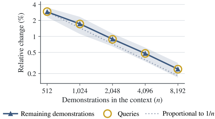
Figure 5: Relative change \rho_{ij} of the TabICL representations when one demonstration is removed, against the number n of demonstrations in the context, on logarithmic axes. The markers show the mean over the four datasets of the per-dataset median, as in Table 5, and the band one standard deviation for the remaining demonstrations. The change of the queries coincides with that of the remaining demonstrations, and both follow the dotted line, which decreases as 1/n .
