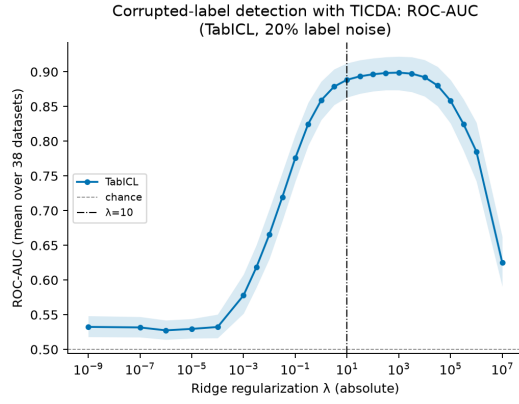
(b) Labeling error detection sensitivity to \lambda .
