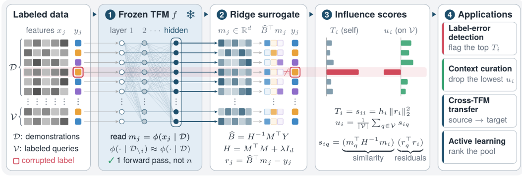
Figure 1: TICDA overview. TICDA (1) extracts TFM embeddings, (2) trains a linear surrogate on the classification task of interest, (3) estimates influence score based on the surrogate and (4) can be applied for label-error detection, context curation, cross-TFM transfer and active learning.
