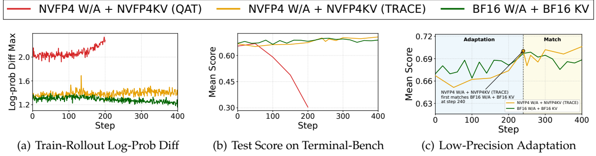
Figure 1: Training dynamics of Qwen3.8-Flash-Next under FP4 rollout. Conventional FP4 QAT exhibits increasing train-rollout discrepancy and degraded test score on Terminal-Bench 2.1, while TRACE maintains stable alignment and enables the policy to progressively adapt to FP4 rollout.
