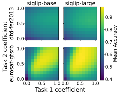
Figure 2: Performance landscapes across model scales. We visualize mean accuracy over a grid of merging coefficients. The heatmaps show highly similar distributions, indicating that the overall shape of the performance landscape is preserved across different model sizes.
