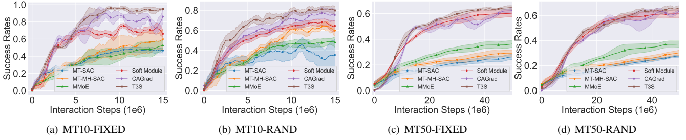
Fig. 4. Training curves of our proposed framework T3S and other baselines on MT10 and MT50 (shaded areas represent the standard deviation over 3 seeds). We plot the average success rate for all tasks on the y-axis, while the x-axis denotes the number of times the multi-task agent interacts with the environment.
