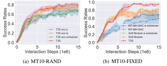
Fig. 7. (a) Ablation study on the task scheduler at MT10-RAND. (b) Ablation study on the feature selector at MT10-FIXED, while analysing several baselines combined with the task scheduler.
