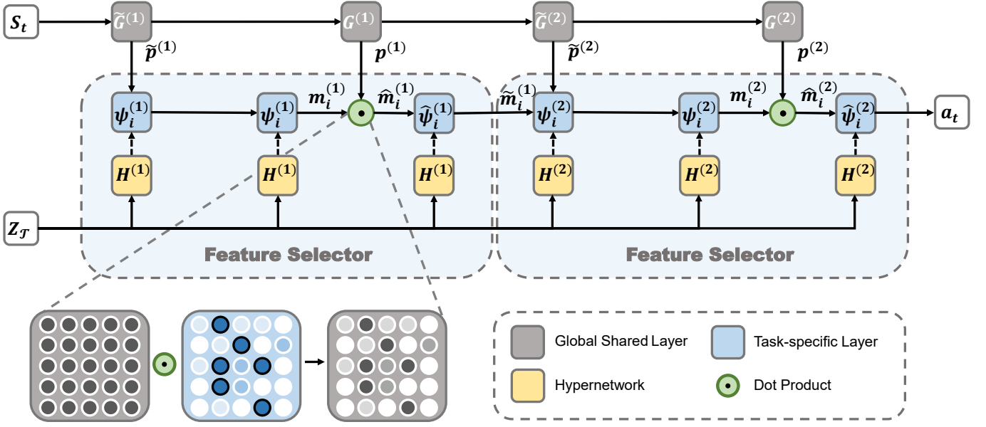
Fig. 2. Visualisation of our network architecture, showing the globally shared network and feature selectors respectively. The role of the feature selectors is to extract task-specific features from the globally shared network using the soft masks. The number of feature selectors can be defined according to the task complexity. Here the solid line (black) denotes the data flow, and the dashed line (black) denotes the weights flow.
