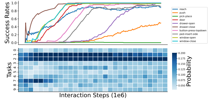
Fig. 5. Sampling history of the task scheduler. (Top: line plot) The success rate for each task in MT10-RAND environment. The x-axis denotes the number of samples during training. (Bottom: square tiles) The sampling history of each task. Each tile represents the probability of sampling over a period, where darker colors denote higher probability.
