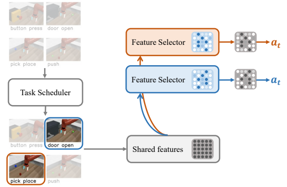
Fig. 1. Overview of our framework T3S. To balance the task difficulty, the task scheduler first selects challenging tasks for the multi-task agent from the whole task set based on the performance metric. Then the feature selector learns which features to be shared between tasks and which not, by filtering task-specific features from globally shared features in an end-to-end manner.
