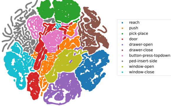
Fig. 6. Visualization of soft masks for different tasks in MT10-RAND. We rollout different tasks and extract the masks from the policy. All masks are grounded in different clusters using t-SNE.
