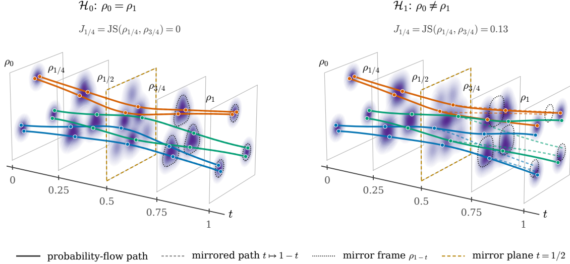
Figure 1: Time reflection of a stochastic interpolant built directly between \rho_0 and \rho_1 using our construction with the linear schedule x_t = (1 - t)x_0 + tx_1 + \sigma t(1 - t)z , \sigma = 1.5 and Gaussian z . Slices show the exact marginals \rho_t . Solid curves are probability-flow paths from six starting points in \rho_0 , coloured by their starting mode; dashed curves mirror the first half of each path under t \mapsto 1 - t , and dotted contours on the slices t = 3/4 and t = 1 outline the mirror frames \rho_{1/4} and \rho_0 . Top: under \mathcal{H}_0 , \rho_t = \rho_{1-t} (Theorem 3.2), each mirrored distribution coincides with the actual one. Bottom: under \mathcal{H}_1 , the mirrored paths end in the outline of \rho_0 while the actual paths end in \rho_1 . All densities and velocity fields are exact Gaussian-mixture expressions; nothing is learned.
