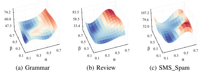
Fig. 4. Hyperparameter sensitivity analysis of token-level AUROC.
