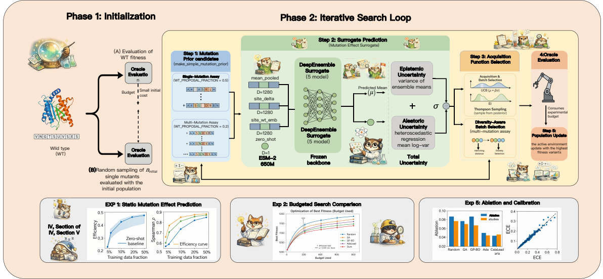
Figure 1: Overall pipeline of Subspace-Guided Evolutionary Search (SGES). SGES starts from the wild-type sequence and a small initial oracle budget, constructs mutation candidates, extracts mutation-aware PLM features, and performs iterative search through surrogate prediction, uncertainty-aware acquisition, oracle evaluation, and population update. This overview connects the representation-level discovery in Section 3 with the search algorithm introduced later: fitness prediction is not treated as generic high-dimensional embedding regression, but is guided by mutation-induced representation changes that expose a compact fitness-relevant structure.
