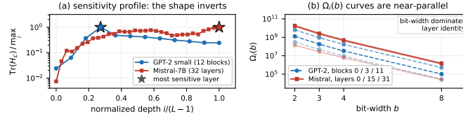
Figure 2: Sensitivity criterion across both models. (a) Hessian trace per layer, normalized by each model’s maximum, against normalized depth; stars mark the most sensitive layer. The profile is strongly non-uniform in both models ( 41\times spread on GPT-2, 135\times on Mistral) but its shape inverts with architecture. (b) The sensitivity tables \Omega_i(b) of equation 6 are near-parallel in both models — a shared, steep sub-4-bit cliff — so bit-width dominates layer identity by orders of magnitude.
