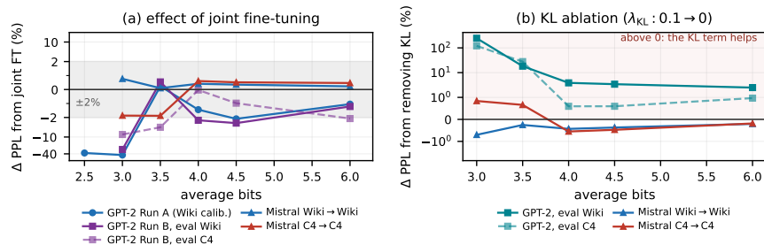
Figure 4: Joint fine-tuning across models, corpora and budgets, on symmetric-log axes so that both the low-bit and near-lossless regimes are legible. (a) Relative perplexity change from adding the joint STE stage to the same allocation; negative is better, shaded band \pm 2\% . Gains are large exactly where quantization damage is large and shrink to a few percent in the usable regime, where the sign becomes model- and corpus-dependent. (b) The KL ablation, \lambda_{KL} : 0.1 \rightarrow 0 : on GPT-2 removing the term is harmful at every budget on both corpora, catastrophically so below 4 bits; on Mistral, where the stage moves far less, the effect is within \pm 1\% and changes sign.
