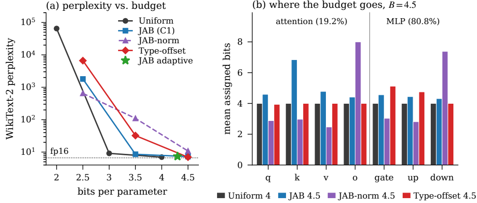
Figure 6: Full-model quantization of Mistral-7B. (a) Perplexity against bits per parameter, GPTQ only. At B = 4.5 Type-offset is best; the adaptive JAB arm (*) spends 4.3 bits per parameter yet scores worse than uniform 4-bit. (b) Mean assigned bits per unit kind at B = 4.5 . Type-offset is flat within a role and offset between roles; JAB over-buys k_proj , which grouped-query attention makes cheap; JAB-norm assigns 8 bits to every o_proj while starving q , k , v to 2–3 bits.
