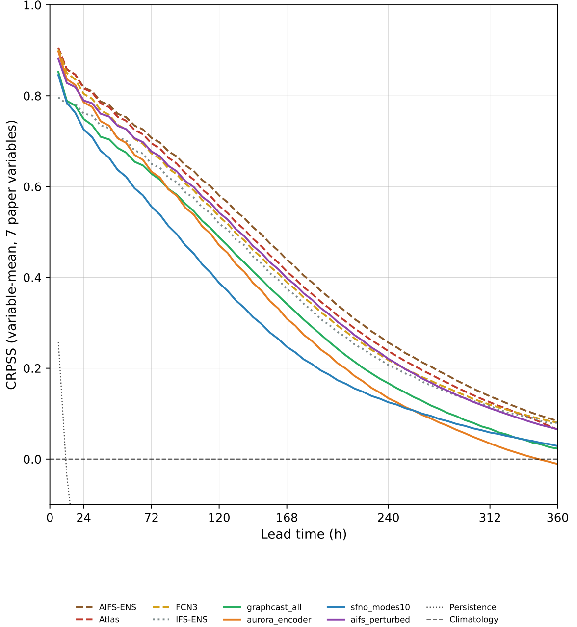
FIG. 3. CRPSS at lead times of 6–360h on the 112-init production grid, variable mean over the seven paper variables (3D variables averaged over 500 and 850 hPa). Solid: SPW (this work); dashed: TP; dotted: the classical IFS-ENS reference. The dashed black line at 0 is the WeatherBench-2 probabilistic climatology; persistence (shown for reference) dives below the -0.1 axis cut after the first two lead times. The IFS-ENS forecasts carry WeatherBench-2 archive NaN gaps in all seven variables, handled by skipna averaging. Per-lead time values and gaps are quoted in the text and Tab. B2.
