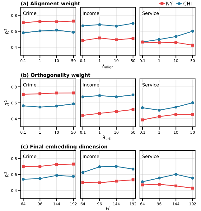
Fig. 4: Impact of (a) alignment weight \lambda_{\text{align}} , (b) orthogonality weight \lambda_{\text{orth}} , and (c) final embedding dimension H , on NYC and CHI. Each curve reports per-task R^2 \uparrow .
