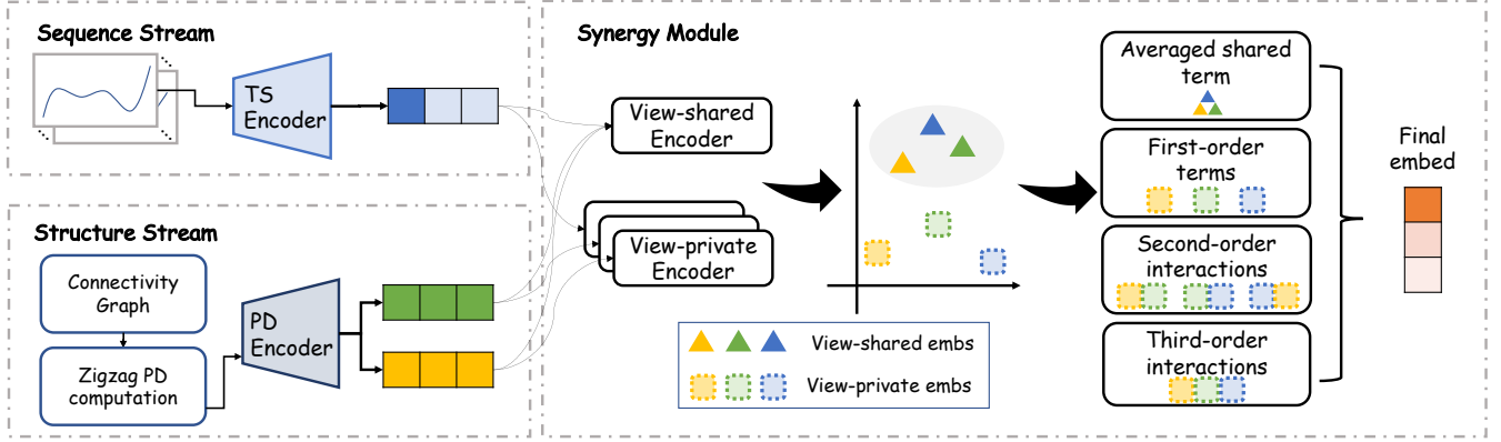
Fig. 2: Overview of MoSS. Left. Two complementary streams encode each region’s mobility. The Sequence (TS) view (top) feeds the per-region hourly inflow/outflow series into a temporal convolutional encoder (TS Encoder), and the Structure (PD) view (bottom) constructs the region-centric connectivity-graph at each time step, computes its zigzag persistence diagram, and encodes the diagram with a permutation-invariant set encoder (PD Encoder). The structure encoder produces source- and destination-side view embeddings. Right. The synergy module fuses the three views. It first applies a shared-private decomposition that factors each view into a cross-view shared embedding (filled triangles) and a view-private embedding (dashed circles), and then aggregates the resulting embeddings through multi-degree interaction that captures first-order, second-order, and third-order interactions in a single per-region embedding.
