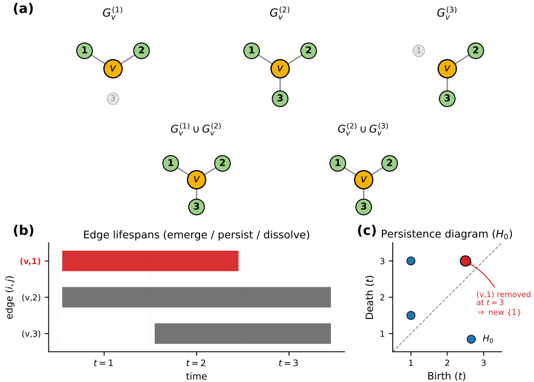
Fig. 3: Structure stream: from a temporal sequence of connectivity-graphs to a persistence diagram. (a) Connectivity-graph G_v^{(t)} at three consecutive time indices (top row), and the union graph G_v^{(t)} \cup G_v^{(t+1)} between every consecutive pair (middle row); filled green nodes are neighbors active at that time, faded gray nodes are inactive. (b) Per-edge lifespans across the window. The bar segments mark the time indices at which the edge is present, exposing the emerge / persist / dissolve dynamics that no single snapshot captures. (c) The resulting zigzag persistence diagram with H_0 features; the diagonal marks zero lifespan.
