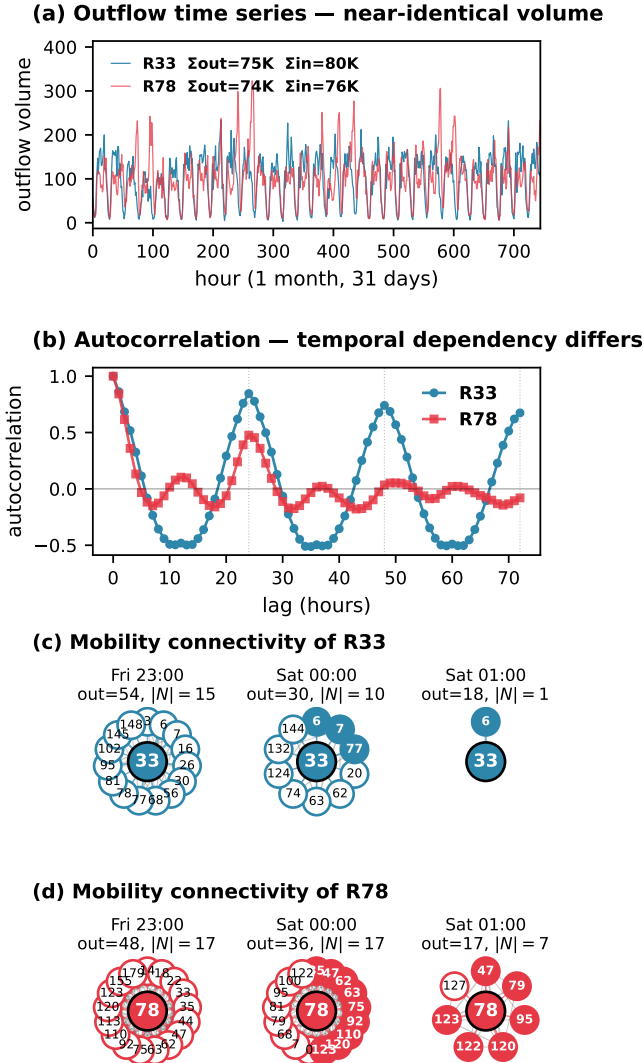
Fig. 1: Same volume, different connectivity dynamics. Two Manhattan regions, R_{33} and R_{78} , with near-identical aggregate mobility over the 31-day study period. (a) Outflow time series over the full month: the two regions are comparable in aggregate volume. (b) Autocorrelation up to a 72 h lag: R_{33} exhibits a strong 24h periodicity while R_{78} shows a much weaker oscillation — their temporal dependency structures differ markedly. (c, d) Inter-region connectivity at three consecutive hours (Fri 23:00 \rightarrow Sat 01:00) over which the two regions also share similar hourly outflow (54/48 \rightarrow 30/36 \rightarrow 18/17 trips). Despite this volume parity, neighborhood dynamics diverge sharply. Solid nodes denote neighbors persistent from the previous snapshot; outlined nodes are new entrants.
