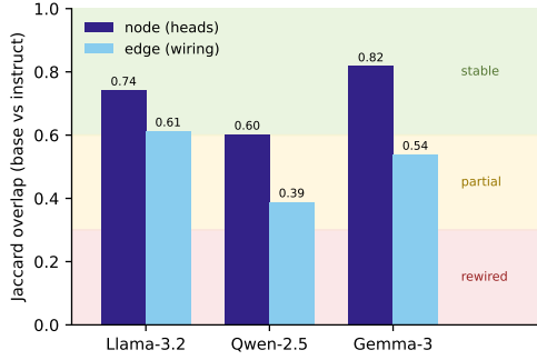
Figure 4: Node (head) vs. edge (wiring) overlap, base vs. instruct. All nodes are in the “stable” band (gating); Llama’s wiring is also stable (strict gating), while Qwen and Gemma drift into “partial” without reaching “rewired”.
