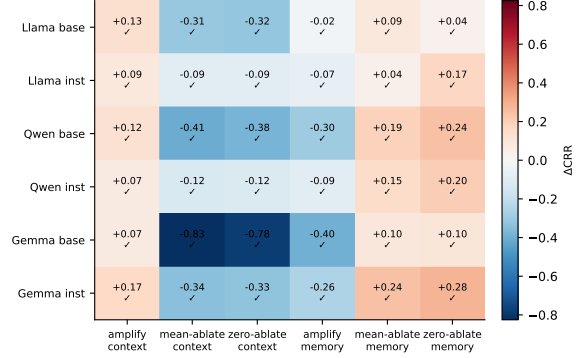
Figure 5: Causal ablation. \Delta\text{CRR} for six interventions across six model variants; ✓ marks a match to the a-priori sign (36/36). Each column is an intervention on a head set: we amplify (scale up), mean-ablate (replace activations with their mean, a soft knock-out), or zero-ablate (set to zero, a harsher knock-out) either the top context heads or the top memory heads, then re-measure CRR.
