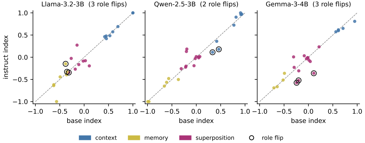
Figure 3: Per-head superposition index, base ( x ) vs. instruct ( y ). Points hug the diagonal (roles stable); ringed points are the 2–3 heads that flip role.
