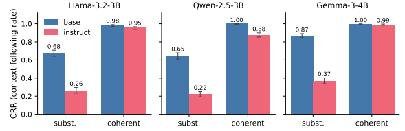
Figure 2: CRR base vs. instruct across families and conflict forms. The tuning effect is large under terse substitution and nearly vanishes under a coherent passage.
