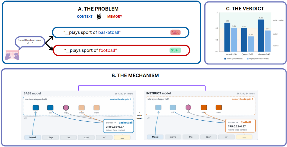
Figure 1: Instruction tuning gates the knowledge-conflict circuit rather than rewiring it. (A) Under a conflict prompt, the model must arbitrate between a false fact injected in context ( basketball ) and the true fact stored in its weights ( football ). (B) The same later-layer context, memory, and superposition heads carry the decision in both base and instruct variants. All head identity, role, and layer position are preserved; only their gain changes. Tuning reweights this fixed set memory-ward, dropping contextual reliance (CRR) from 0.65–0.87 in base models to 0.22–0.37 in their instruct siblings under terse substitution conflict. (C) Across all three families, base-vs-instruct node (head) overlap sits in the stable band ( J = 0.60\text{--}0.82 ), with edge overlap equal or lower (0.39–0.61) but never reaching the rewiring threshold. Hence, we label Llama as strict gating and, Qwen and Gemma as gating with an ambiguous edge sub-type.
