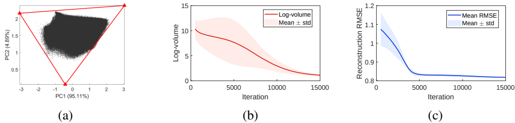
Fig 3: Estimation results for the Geology-1 scene, averaged over 20 independent replications. (a) Projected data cloud (first two PCs, 95.11% and 4.89% of variance) and the simplex of the mean estimated vertices. (b) Log-volume and (c) reconstruction RMSE versus training iteration (mean \pm 1 standard deviation).
