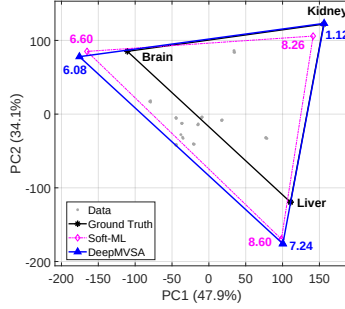
(a) Projection of the micro-array data onto the first two PCs, which explain 47.9% and 34.1% of the total variance.
