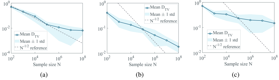
Fig 1: Total-variation distance D_{TV}(\mathbb{P}_{\mathcal{S}_T}, \mathbb{P}_{\mathcal{S}}) versus sample size N on synthetic simplices for K = 3, 5, 7 (log-log axes). Solid curves: mean over 20 independent replications; shaded bands: \pm 1 standard deviation. Dashed line: the N^{-1/2} reference rate of Theorem 3.1.
