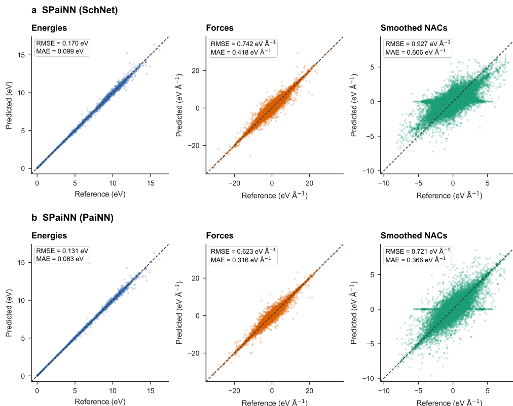
Supplementary Fig. 3. Static test predictions of SPaiNN models for \text{CH}_2\text{NH}_2^+ . SPaiNN 1 models use a , SchNet 12 and b , PaiNN 13 architectures. Columns show predicted versus MR-CISD/aug-cc-pVDZ reference energies, Cartesian force components and SNAC components. Both models use validation-selected checkpoints and the same 1,250 held-out test geometries as Supplementary Fig. 2 . Insets report MAE and RMSE.
