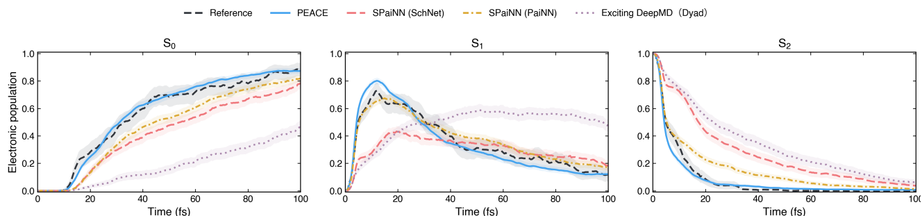
Supplementary Fig. 4. \text{CH}_2\text{NH}_2^+ population dynamics. Reference S_0 , S_1 and S_2 populations are compared with PEACE, SPaiNN–SchNet, SPaiNN–PaiNN 1 and Exciting DeePMD Dyad 14 over 100 fs. The four machine-learning methods use the same 1,000 initial geometries and velocities, with trajectories initiated in S_1 . Independent selection for complete trajectories with a maximum absolute total-energy drift below 0.25 eV retains 947, 418, 758 and 453 model trajectories, respectively. Shading indicates pointwise 95% confidence intervals from trajectory-level bootstrap resampling 16 .
