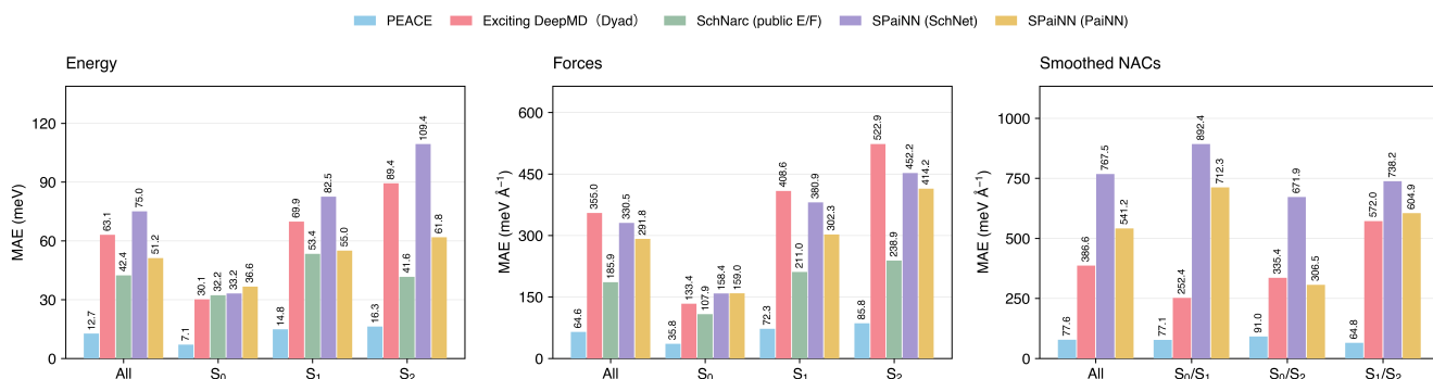
Supplementary Fig. 5. Unseen 770-geometry \text{CH}_2\text{NH}_2^+ benchmark. Energy, force and SNAC MAE are evaluated on the same 770 geometries from the SchNarc benchmark 7 . Comparisons include PEACE, Exciting DeePMD 14 , SchNarc 7 and SchNet- and PaiNN-based SPaiNN models 1 . Force and SNAC errors are averaged over Cartesian components. Each predicted SNAC vector was sign-aligned independently for each geometry and state pair by choosing the sign that minimized its error relative to the reference vector. The public SchNarc 7 checkpoint has no NAC prediction head, so no SNAC error is reported.
