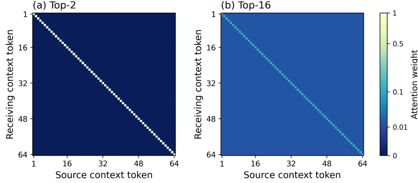
Figure 12: The learned context-attention structure depends strongly on the aggregation target. The context-attention matrix A_1 is (a) sharply concentrated on the diagonal for top-2 task, but (b) distributed broadly across context tokens for top-16 task.
