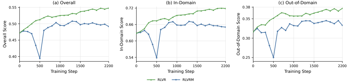
Figure 11 Evaluation performance during RL. We report overall, in-domain, and out-of-domain scores every 100 training steps using CPS with \eta = 0.7 . RLVR shows steady performance improvements, whereas RLVLm soon stagnates. The sudden drop of RLVLm at 400-500 steps is investigated in Sec. B.5.
