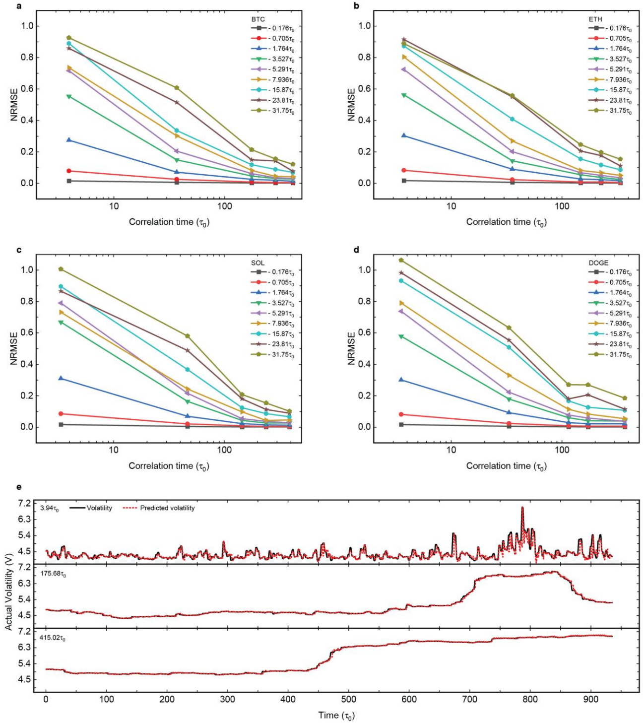
Fig. 3 | Forecasting of cryptocurrency prices volatility: a-d , NRMSE vs volatility correlation time \tau curves for four cryptocurrencies, a , Bitcoin (BTC), b , Ethereum (ETH), c , Solana (SOL) and d , Dogecoin (DOGE) respectively, for a fixed past window size of 15.87\tau_0 and future window sizes of 0.176\tau_0 - 31.75\tau_0 . e , Comparison of the target (solid black line) and predicted (dotted red line) BTC price volatility vs time for a past window size of 15.87\tau_0 and a future window size of 3.527\tau_0 , respectively. The top, middle and bottom plots are for a calculated correlation time of 3.94\tau_0 , 175.68\tau_0 and 415.02\tau_0 respectively. For the values of the averaging window sizes used to obtain relevant correlation times from the volatility data, see Table 1.
