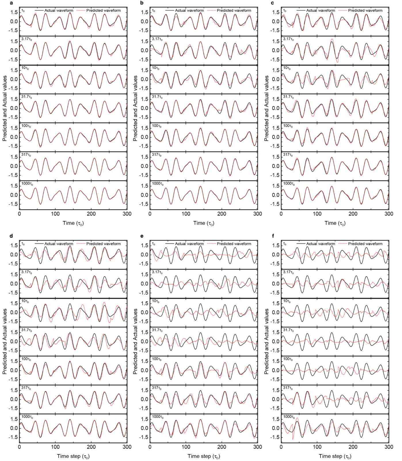
Fig. S2 | Reconstruction of deterministic signal vs time. a-f, reconstruction from different noise levels D = 0.04 (a), 0.127 (b), 0.4 (c), 1.27 (d), 4 (e), 12.7 (f) respectively. The first prediction in each subplot is for the smallest coloured noise correlation time \tau_0 , increasing up to 1000\tau_0 down each subplot. The target signal and reconstructed waveform are denoted by the solid black line and dotted red line respectively.
