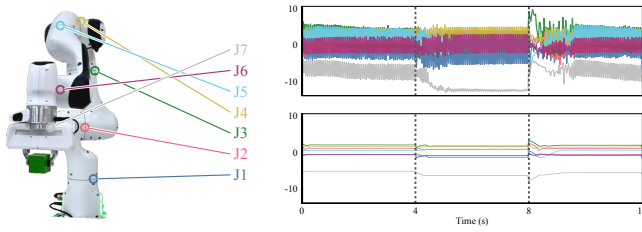
Fig. 5. Franka robot with color-coded joints (left) and corresponding raw policy outputs during Reach (right). After each target change (dashed lines), CATS (bottom) responds with smaller action changes and quickly settles to stable outputs, whereas PPO (top) exhibits larger action changes followed by persistent oscillations.
