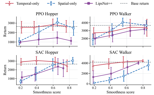
Fig. 2. Return at matched smoothness levels on Hopper and Walker. For each target score in \{0.2, 0.4, 0.6, 0.8\} , we compared configurations whose smoothness scores (lower is better) are within 10% of the target. Error bars indicate 95% confidence intervals.
