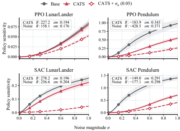
Fig. 4. Next-state-noise extension on LunarLander and Pendulum. R denotes return and sm the smoothness score. Shaded regions indicate 95% confidence intervals.
