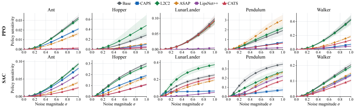
Fig. 3. Policy sensitivity under observation noise for PPO (top) and SAC (bottom). Shaded regions indicate 95% confidence intervals.
