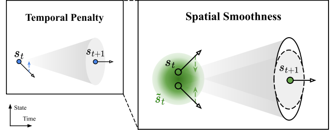
Fig. 1. From temporal regularization to spatial smoothness. Black arrows denote actions; colored arrows indicate alignment. The temporal penalty aligns actions along transitions (left). When nearby states share possible next states, this alignment can indirectly bring their actions closer (right).
