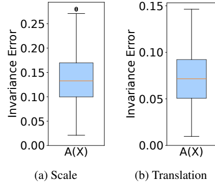
Figure 30: Results for first block of Transformers trained on ShapeNet part centroid prediction with 16 \text{Scale}(3) (left) or \text{T}(3) augmentations (right) per sample. Both attention maps are approximately invariant to the respective group.
