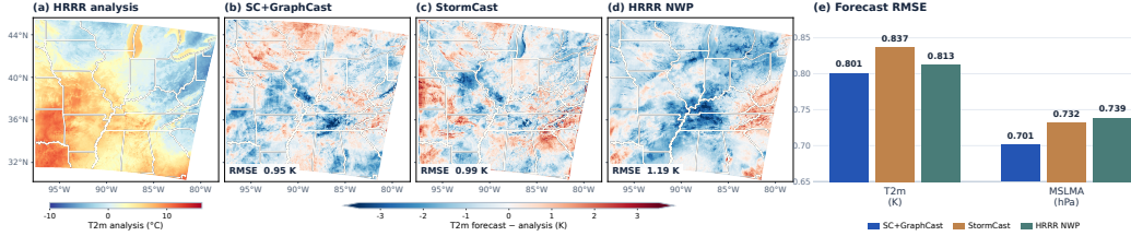
Figure 6: Cross-dataset experiment results. (a) HRRR analysis of 2 m temperature. (b–d) Models' forecasts minus the same analysis. (e) RMSE comparison for T2m and MSLMA.
