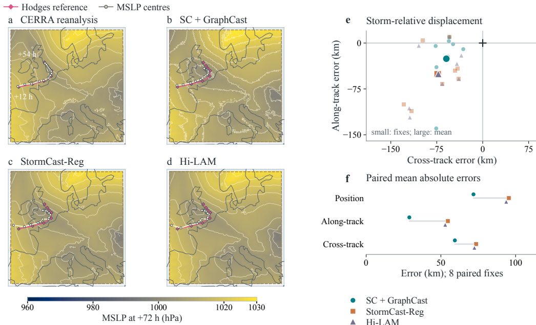
Figure 12: November case and storm-relative displacement. Event 1812, initialized at 00 UTC on 16 November 2022. a–d , MSLP at +72 h and cumulative Hodges and independently tracked field centres. e , Along- and cross-track displacement at eight shared fixes with equal kilometre scales; positive values indicate ahead of and right of reference motion. Large symbols mark means. f , Mean distance and mean absolute displacement components.
