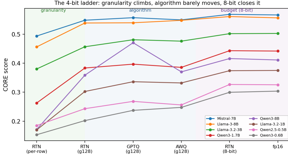
Figure 4: Per-model CORE across the ladder (per-row RTN → g128 RTN → GPTQ → AWQ → 8-bit RTN → fp16). Qwen3-8B’s GPTQ spike above fp16 is the noted 200-sample outlier.
