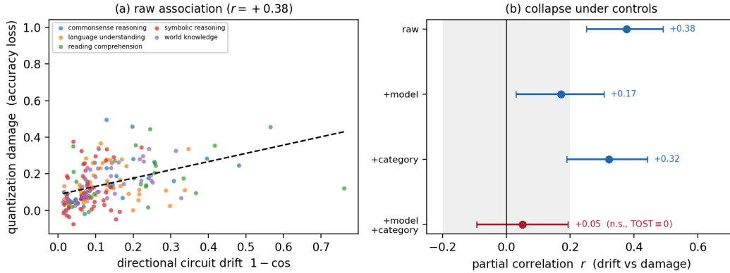
Figure 2: Circuit drift vs. damage. (a) Pooled scatter of drift against damage across 198 (task, model) pairs, with the raw regression line. (b) Partial correlation between drift and damage as controls are added left-to-right (TOST \pm 0.2 equivalence band shaded), ending with model and task category held jointly constant.
