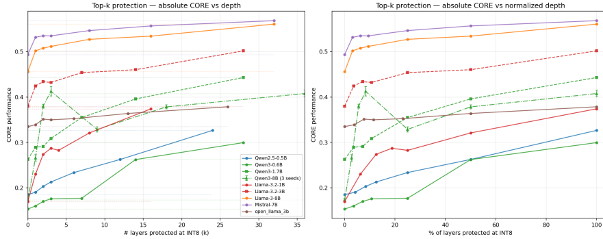
Figure 3: Cumulative CORE as the top- k most-recoverable layers are restored to 8-bit (rest at 4-bit), against each model’s 4-bit (floor) and 8-bit (ceiling) bands. Layers are ranked by their own protect-one recovery, an oracle ordering, not a deployable selector. Curves are absolute CORE on the finite 200-sample subset, so cross-model levels track fp16 baselines (Qwen3-8B’s level sits marginally below Qwen3-1.7B’s here, a small-sample ordering, not a model defect); all claims are within-model recovery. Color=family, marker/linestyle=size.
