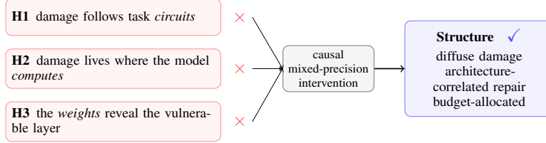
Figure 1: Three hypotheses, one causal test. Three hypotheses for where quantization damage lives (H1–H3, left) are each refuted by mixed-precision intervention (center, \times ); the resulting pattern is shown at right ( \checkmark ).
