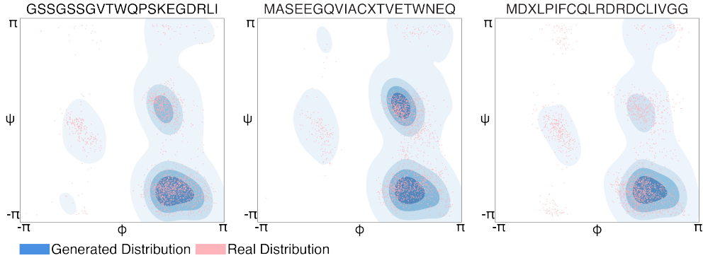
Fig. 6: Torsion angle generation on the torus \mathbb{T}^2 . True and generated distributions of protein backbone torsion angles (\phi, \psi) for held-out mdCATH proteins, conditioned on ESM embeddings of their sequences (first 20 amino acids shown in subplot titles). RWEFM accurately captures the multimodal structure of conformational distributions.
