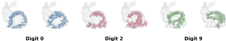
Fig. 5: Distributions generated on the Stanford bunny. RWEFM-generated empirical distributions on a general triangulated mesh with no closed-form geometry, showing two samples per digit class (0, 2, 9). Generated points lie on the curved surface and recover the digit morphology, illustrating RWEFM on arbitrary geometries (Table 3).
