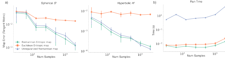
Fig. S2: Entropic Map Benchmark. a. We evaluate our Riemannian entropic map estimator on constructed examples on the sphere \mathbb{S}^2 and hyperbolic space \mathbb{H}^2 where the ground-truth map is known. This ground truth arises from shifting an original distribution via the Riemannian gradient of a convex function over each space. We compare the estimation error against the Euclidean entropic map and the unregularized OT map. b. Computational efficiency of our Riemannian entropic map implementation compared the Euclidean map and solving unregularized OT.
