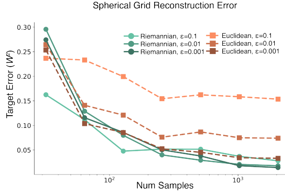
Fig. S3: Entropic map reconstruction error For the spherical grid example from Figure 3, we benchmark the map quality of entropic and euclidean map estimators as a function of sample size and regularization strength. We report the (Spherical) EMD between the source samples pushed forward by the estimated map and the target samples.
