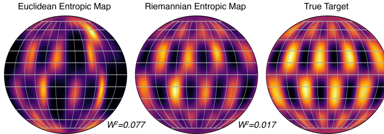
Fig. 3: Riemannian Entropic Map. Gaussian-to-checkerboard transport on \mathbb{S}^2 using Euclidean (left) and Riemannian (middle) entropic maps. The Riemannian approach respects the underlying geometry, resulting in a more accurate mapping (see Figure S2).
