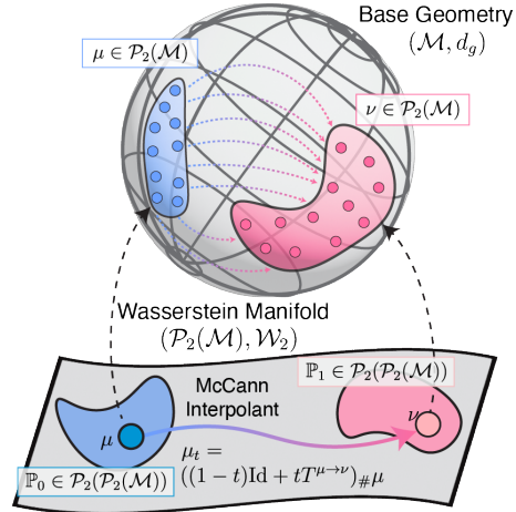
Fig. 1: Riemannian Wasserstein Entropic Flow Matching. Top: Base Riemannian manifold (\mathcal{M}, d_g) . Each blob is a probability distribution \mu, \nu \in \mathcal{P}_2(\mathcal{M}) and a single training example is one blob, not one point. The dashed line is the Riemannian OT path between \mu and \nu which is estimated via point-cloud samples from each blob using the entropic map. Bottom: Wasserstein manifold (\mathcal{P}_2(\mathcal{M}), \mathcal{W}_2) , where a blob is a distribution-over-distributions and each point is a distribution in the top figure. The same dashed path lifts here as the McCann interpolant \mu_t , the geodesic along which RWEFM learns its flow.
