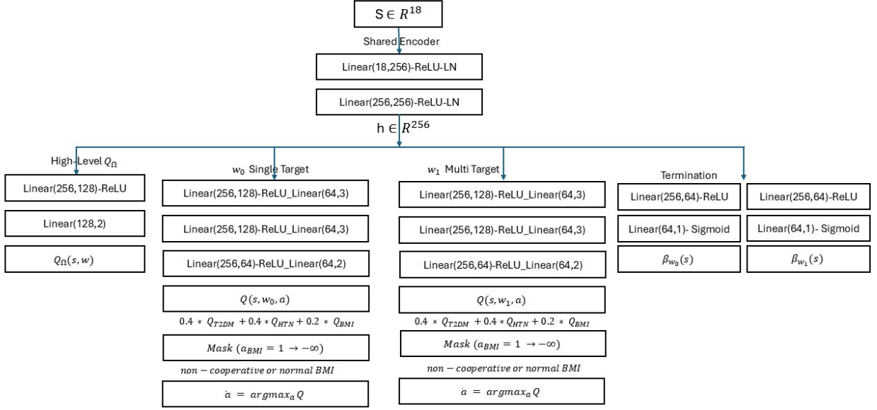
Figure 6: Factored action hierarchical option-critic (FAHOC) framework network architecture. The shared encoder maps state s \in \mathbb{R}^{18} to a 256-dimensional embedding h . Four parameter groups branch from h : the high-level head outputs Q_n(s, \omega) over the two options ( \omega_0 : Single-Target, \omega_1 : Multi-Target); per-option factored heads decompose the intra-option Q-value as Q(s, \omega, a) = 0.4 Q_{t2dm} + 0.4 Q_{htn} + 0.2 Q_{bmi} (Eq. 21); an action mask sets Q(s, \omega, a) = -\infty for a_{bmi}=1 when the patient is non-cooperative or has normal BMI, preventing infeasible treatment selections; and per-option termination heads output \beta_\omega(s) \in (0, 1) via sigmoid. LN = Layer Normalization; \sigma = Sigmoid.
